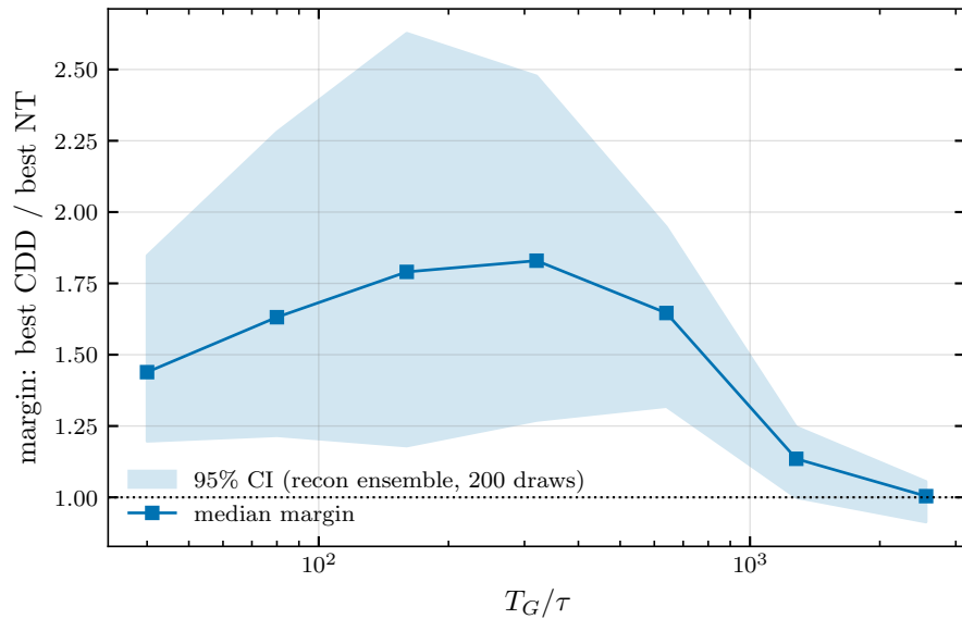
NT advantage under reconstruction uncertainty
