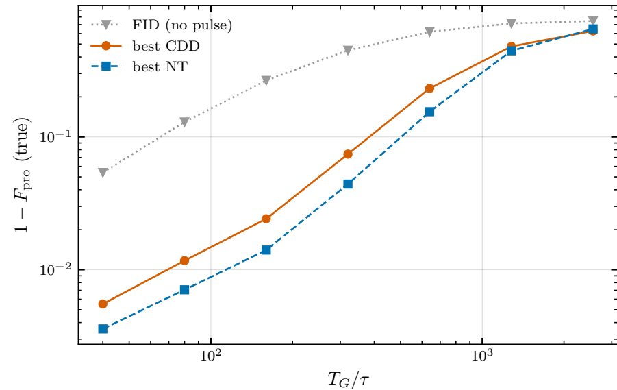
CZ infidelity vs gate time (anchored model)
