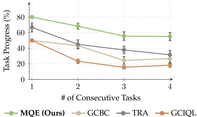
Figure 5: Task progress on BridgeData tasks based on how many consecutive tasks the agent is required to perform, plotted with both the mean and the standard error bars.
