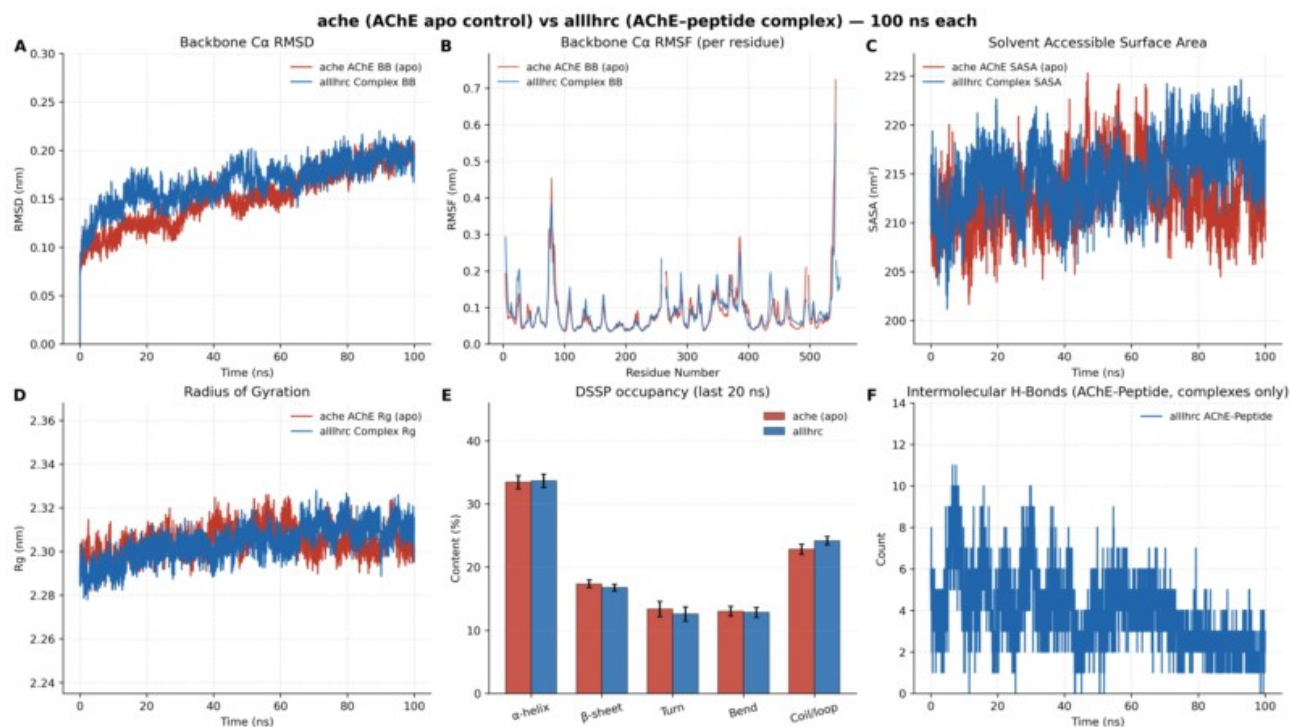
Figure 5. Apo AChE versus AChE-ALLHRC. Panels A–F match Table 7. Complex RMSD (A) tracks apo; hydrogen bonds (F) fall from early occupancy to about two in the last 20 ns.
