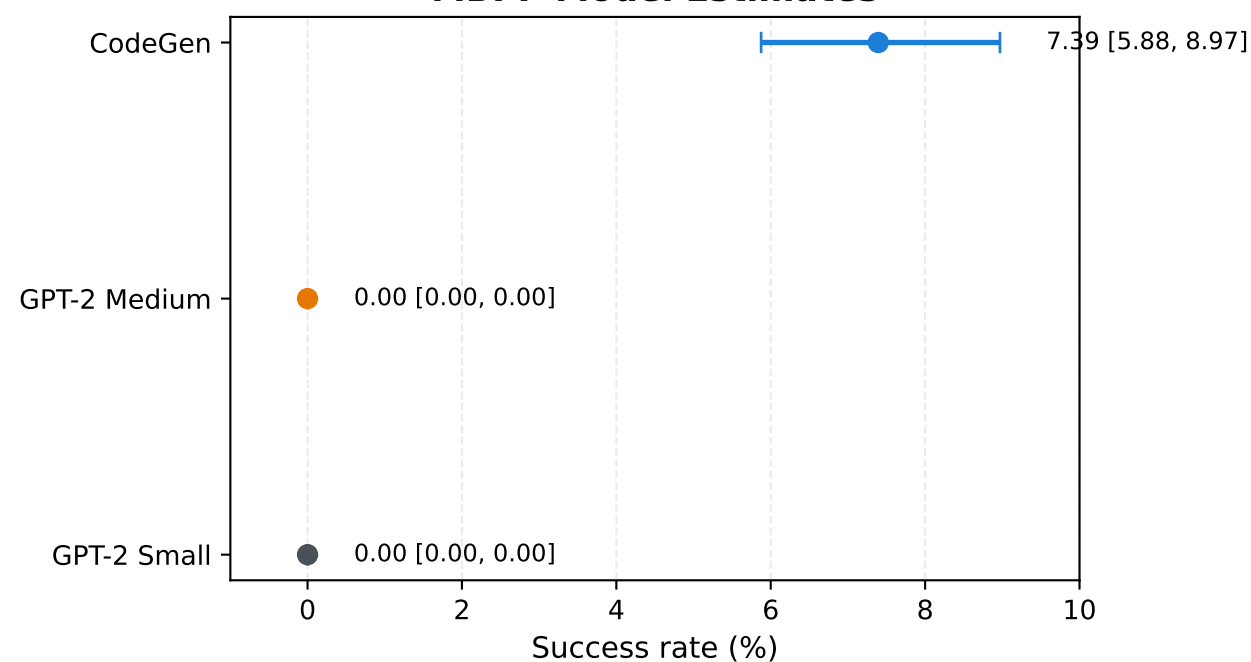
MBPP Model Estimates
