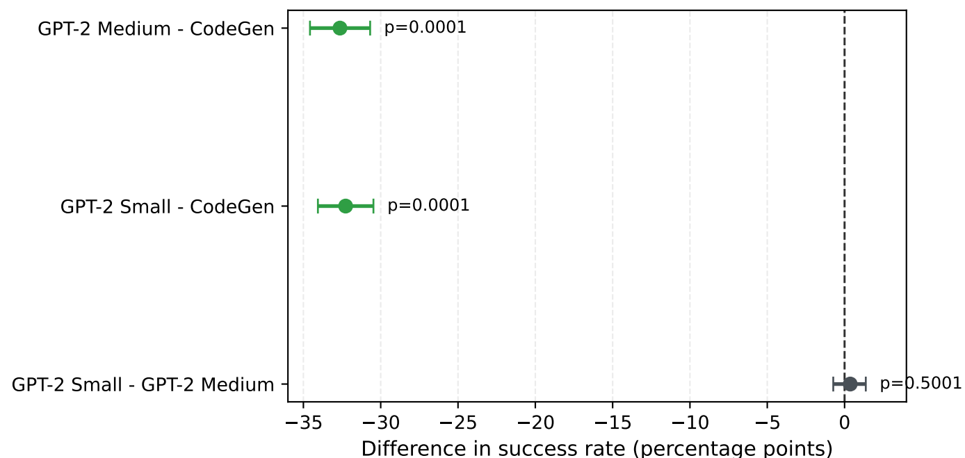
MBPP Pairwise Differences
