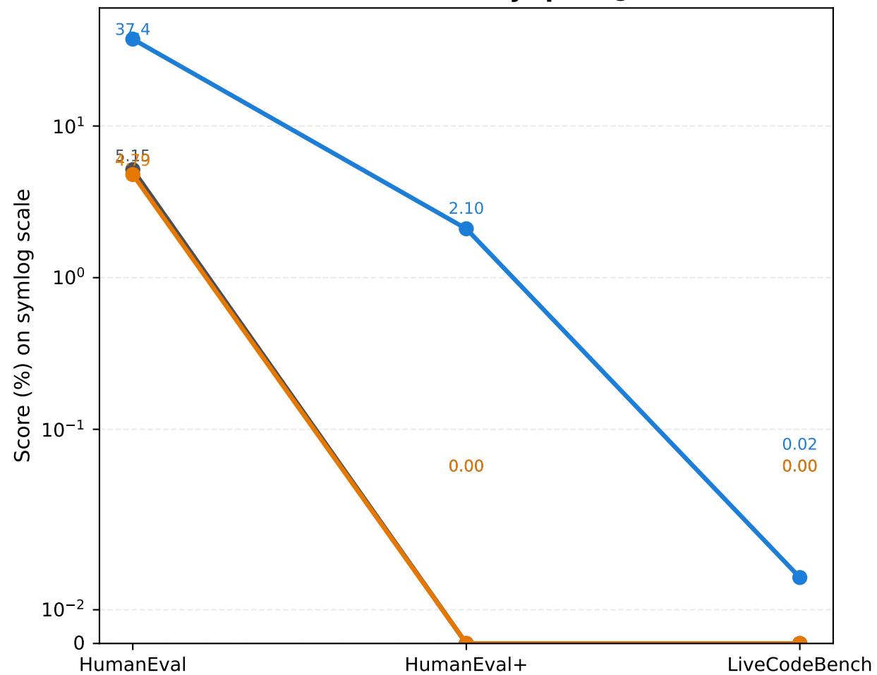
HumanEval Family (pass@1)
