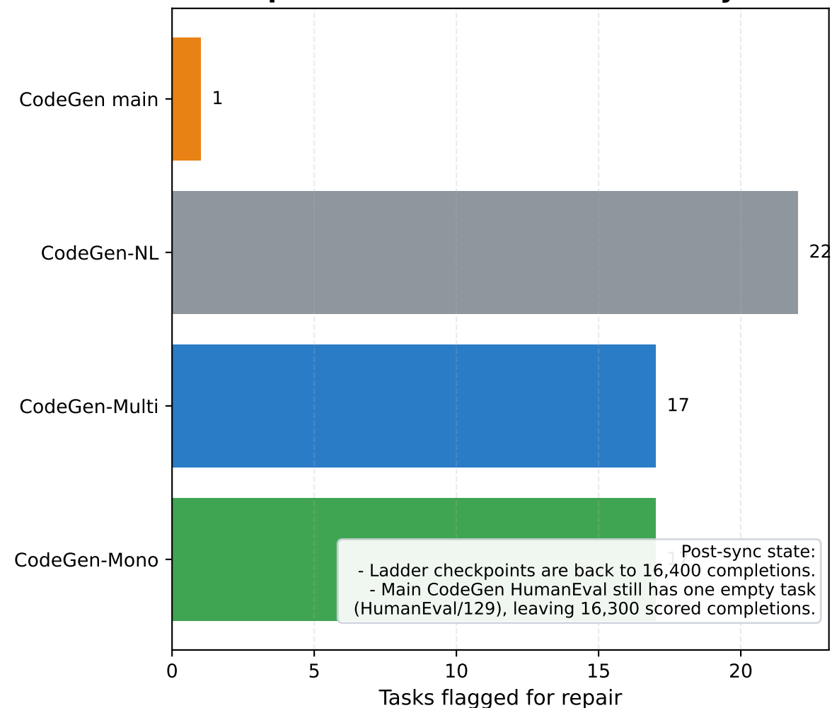
Repair Burden Before the Final Sync
