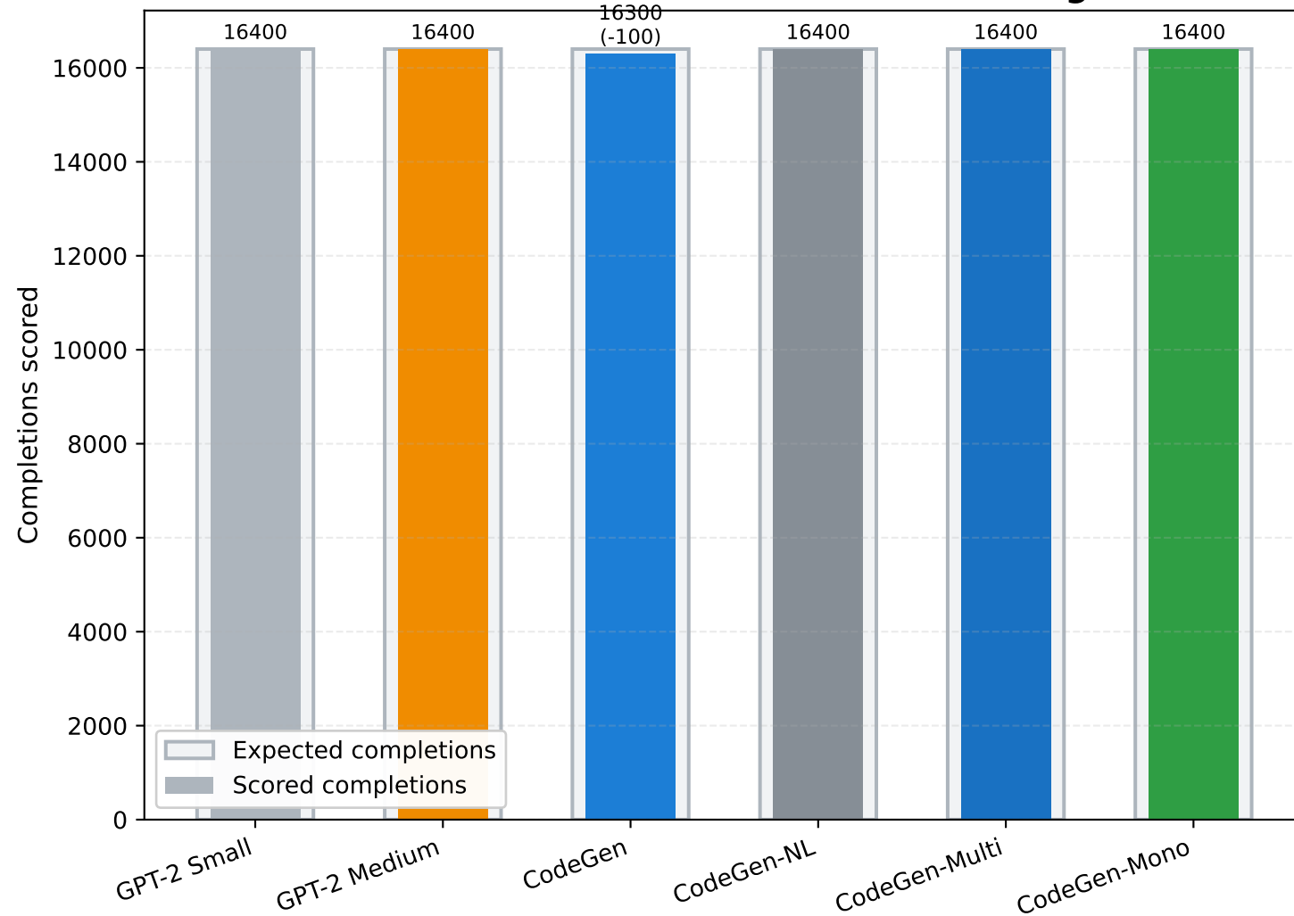
Scored vs Intended HumanEval Coverage
