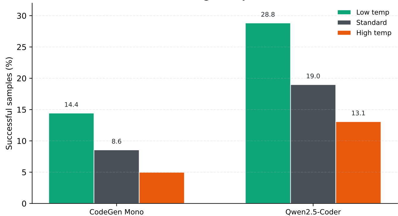
MBPP Decoding: Sample Success
