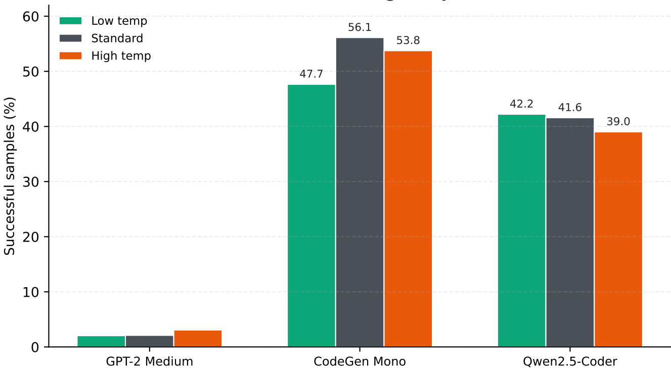
HumanEval Decoding Temperature
