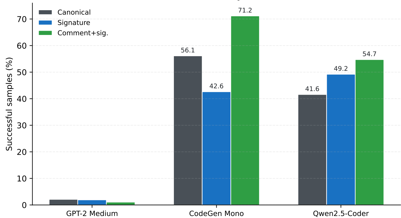
HumanEval Prompt Format
