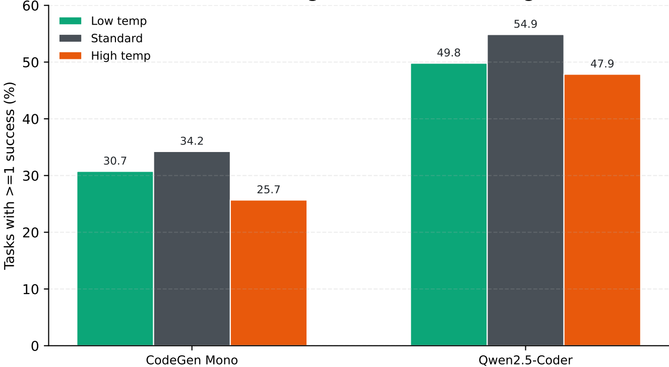
MBPP Decoding: Distinct-Task Coverage
