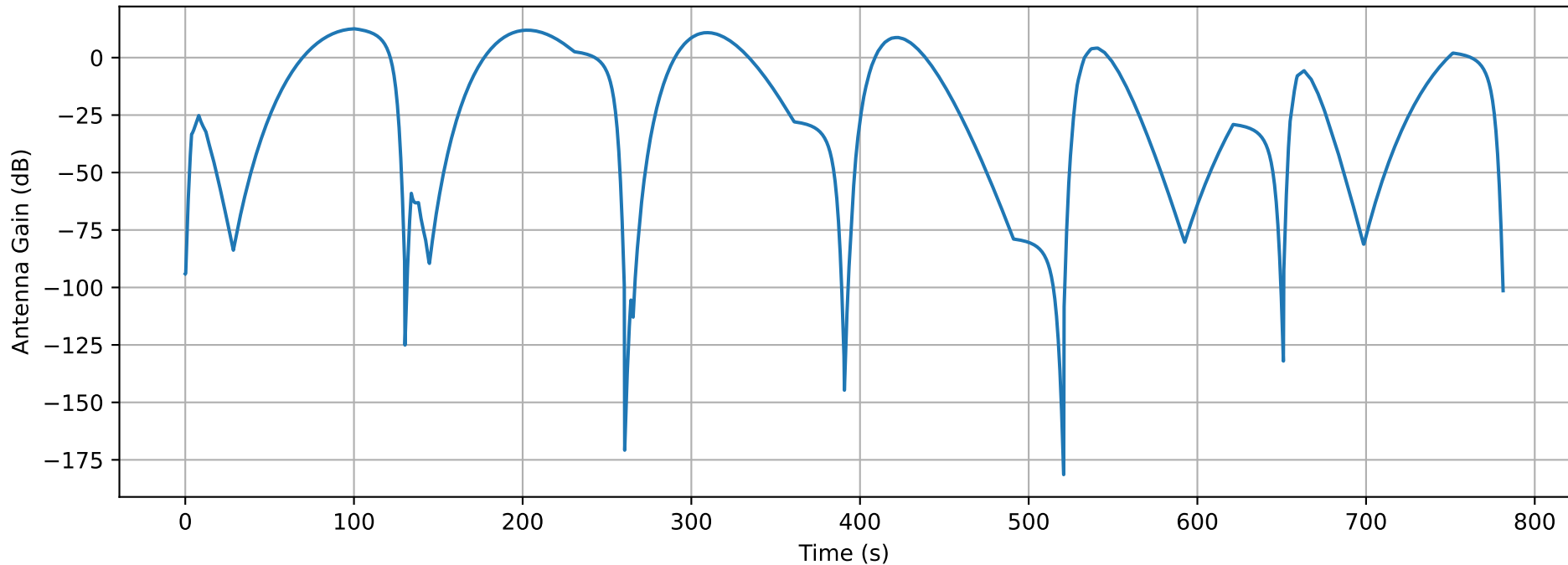
Antenna Gain Along Path — SPIRAL_6orbit_spc15m_alt25m_20260310T141438Z.csv
