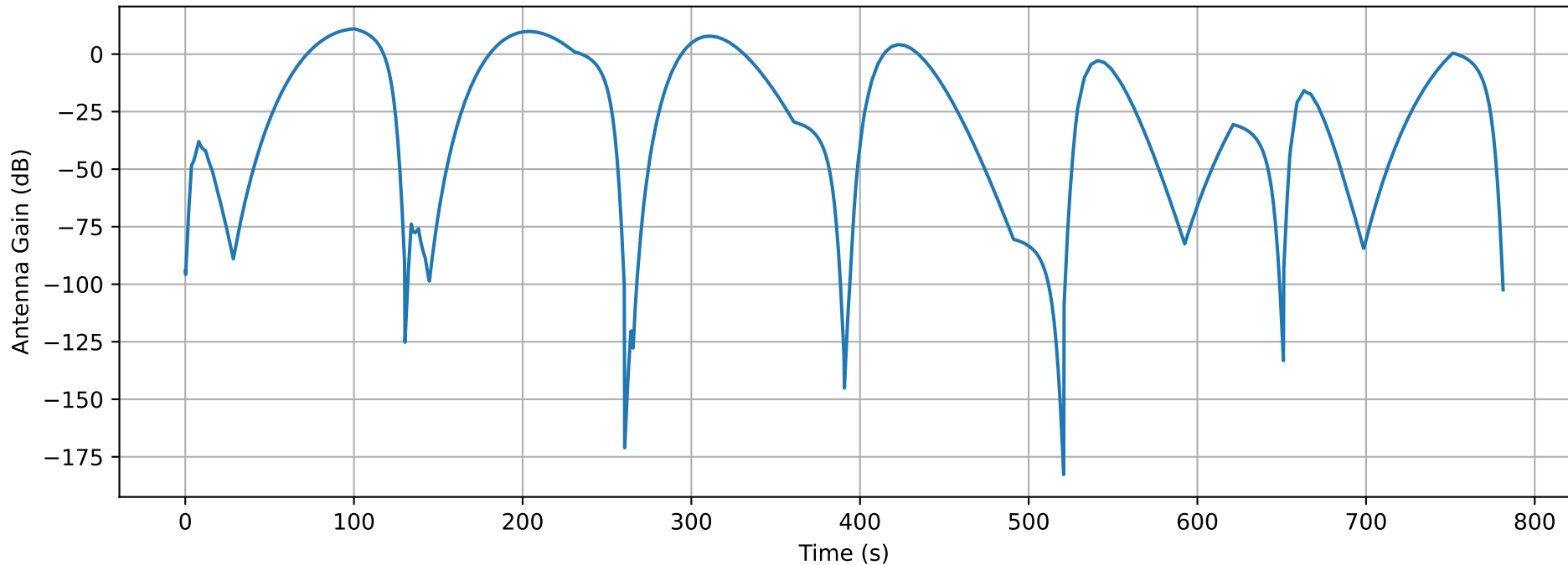
Antenna Gain Along Path — SPIRAL_6orbit_spc15m_alt35m_20260310T141450Z.csv
