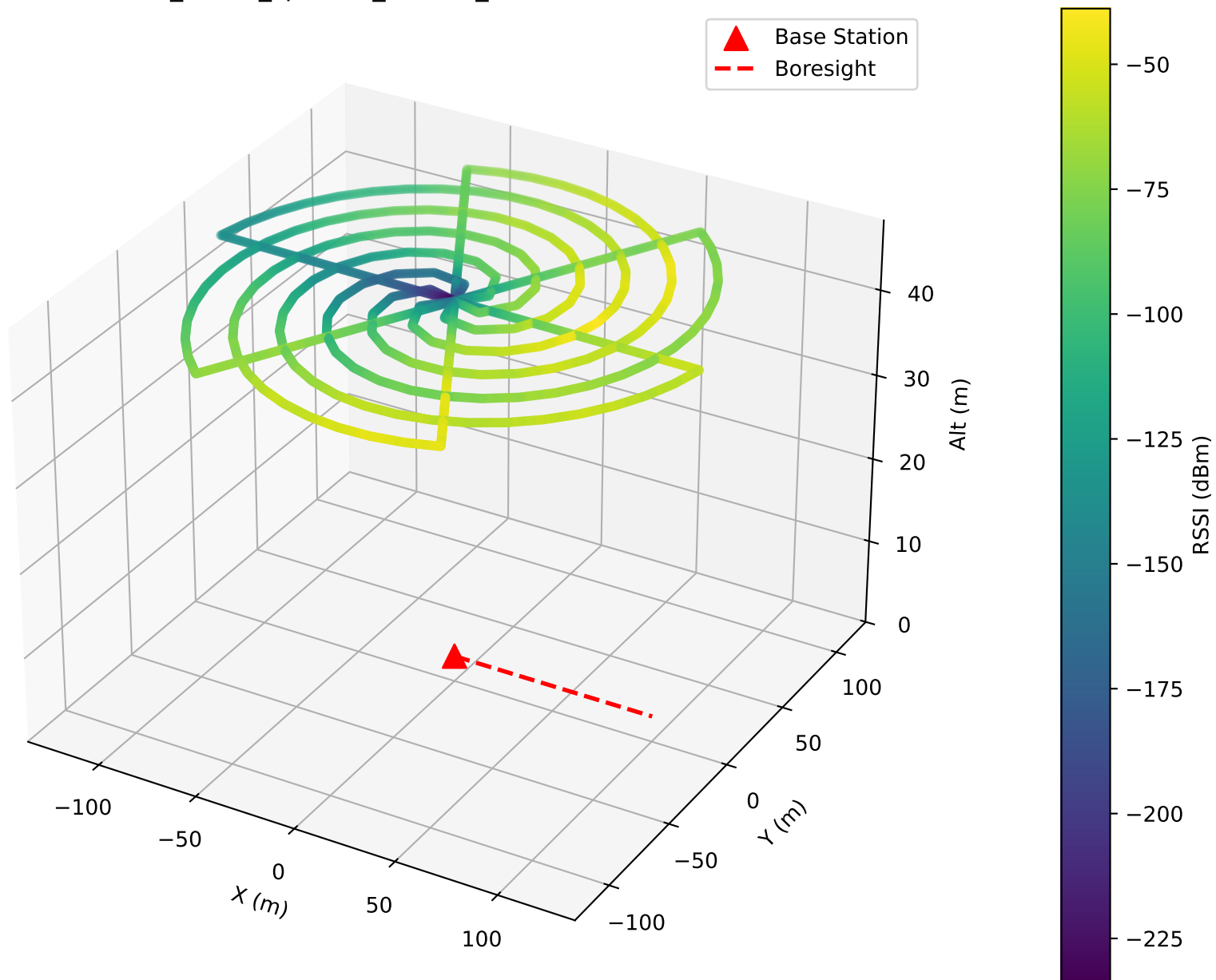
3D Path — RSSI (dBm) SPIRAL_6orbit_spc15m_alt45m_20260310T141500Z.csv
