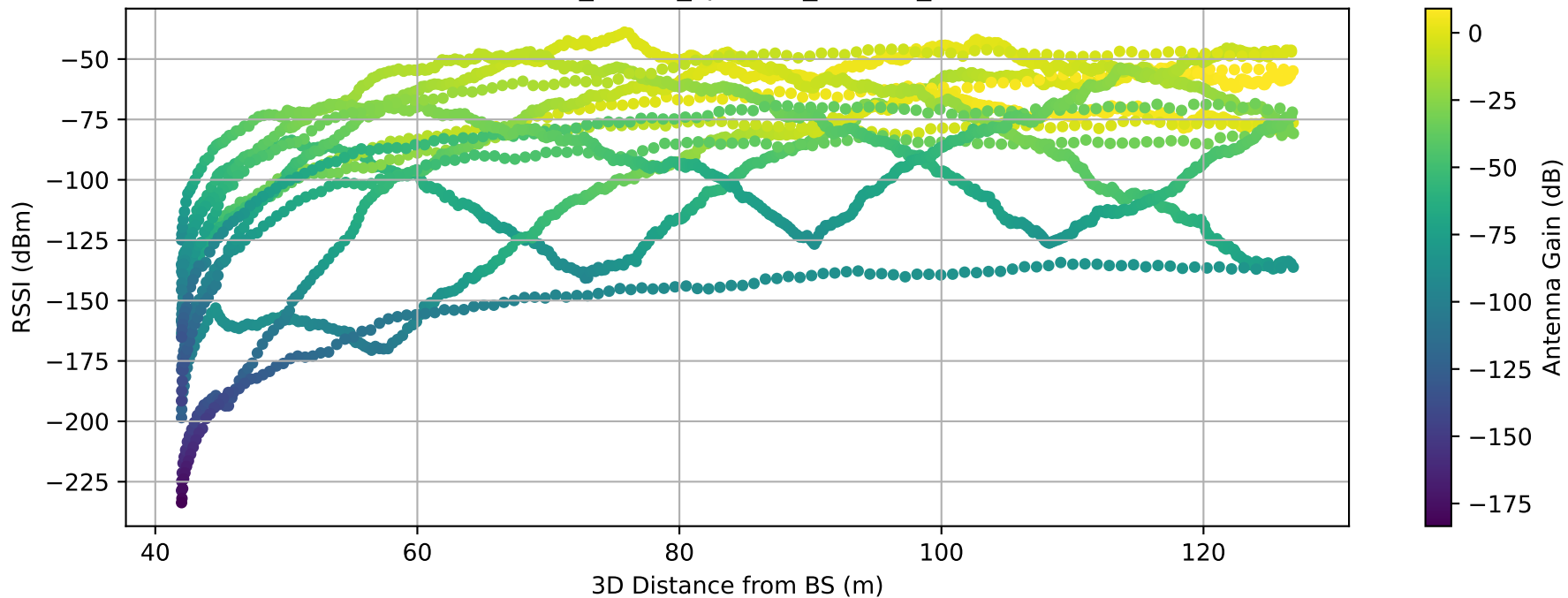
RSSI vs Distance — SPIRAL_6orbit_spc15m_alt45m_20260310T141500Z.csv
