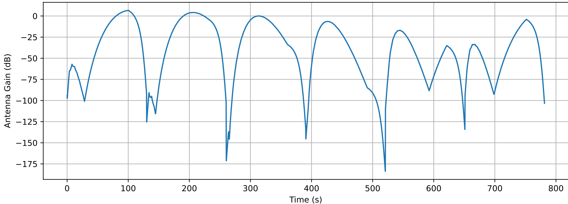
Antenna Gain Along Path — SPIRAL_6orbit_spc15m_alt55m_20260310T141538Z.csv
