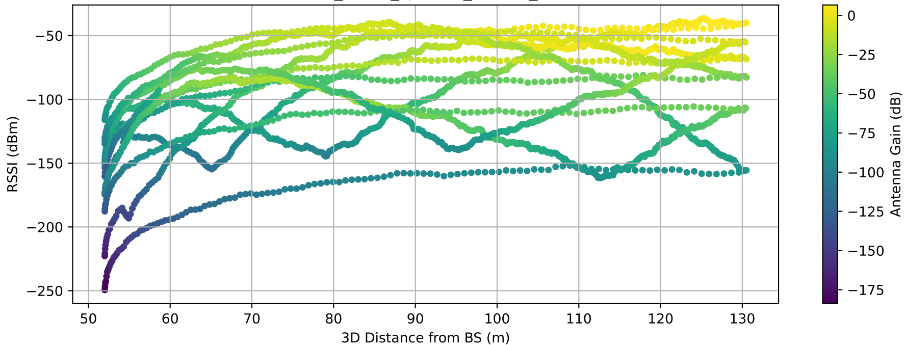
RSSI vs Distance — SPIRAL_6orbit_spc15m_alt55m_20260310T141538Z.csv
