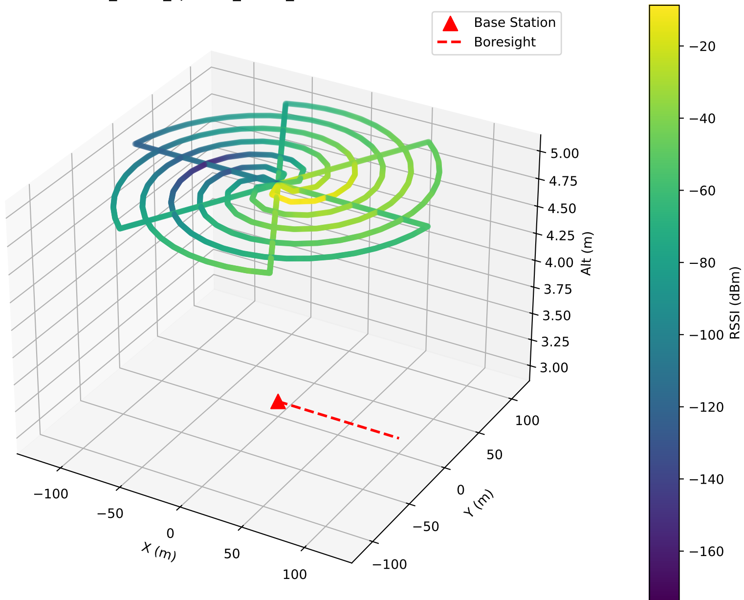
3D Path — RSSI (dBm) SPIRAL_6orbit_spc15m_alt5m_20260310T141402Z.csv
