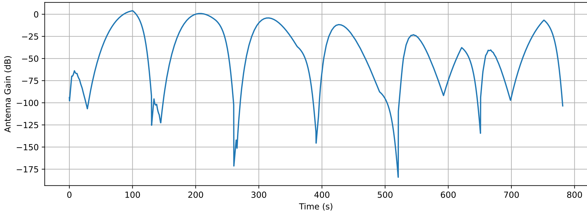
Antenna Gain Along Path — SPIRAL_6orbit_spc15m_alt65m_20260310T142419Z.csv
