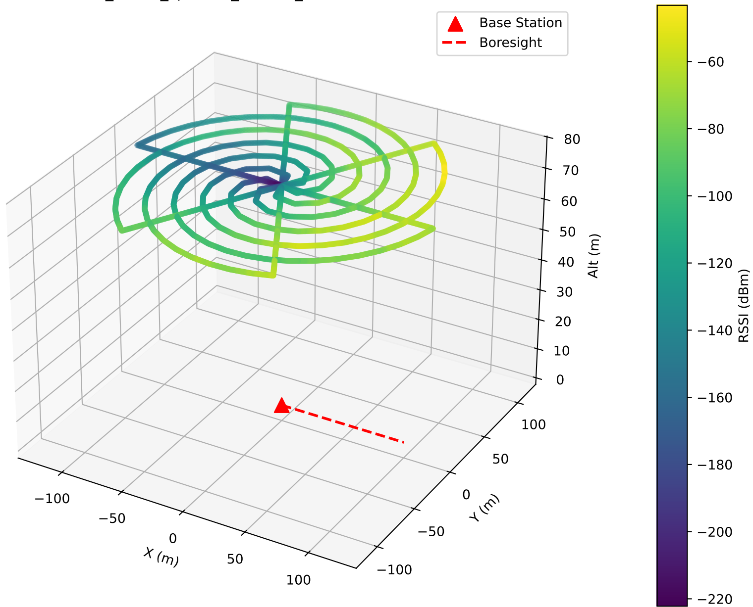
3D Path — RSSI (dBm) SPIRAL_6orbit_spc15m_alt75m_20260310T142430Z.csv
