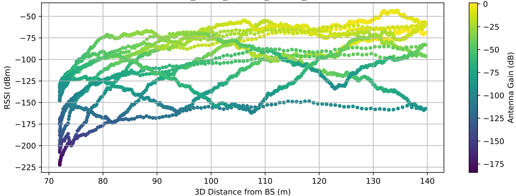
RSSI vs Distance — SPIRAL_6orbit_spc15m_alt75m_20260310T142430Z.csv
