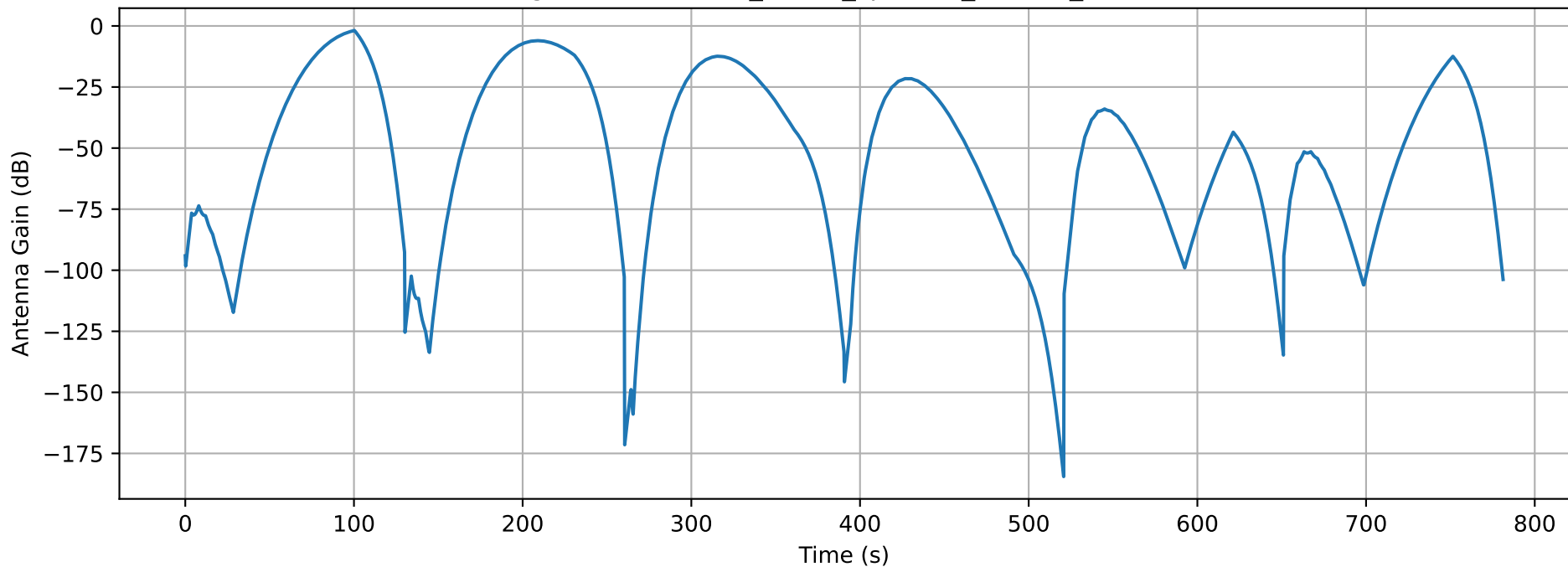
Antenna Gain Along Path — SPIRAL_6orbit_spc15m_alt85m_20260310T142439Z.csv
