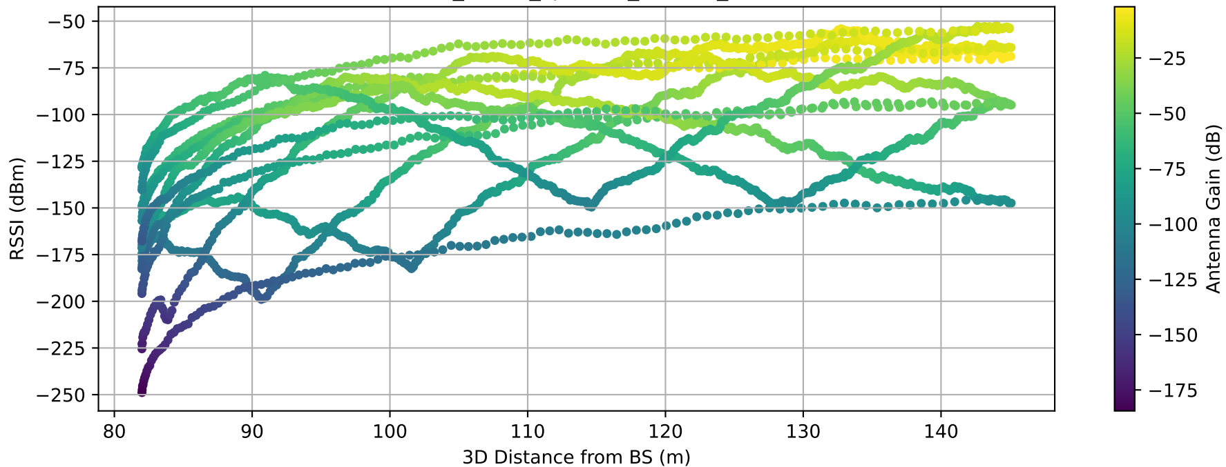
RSSI vs Distance — SPIRAL_6orbit_spc15m_alt85m_20260310T142439Z.csv
