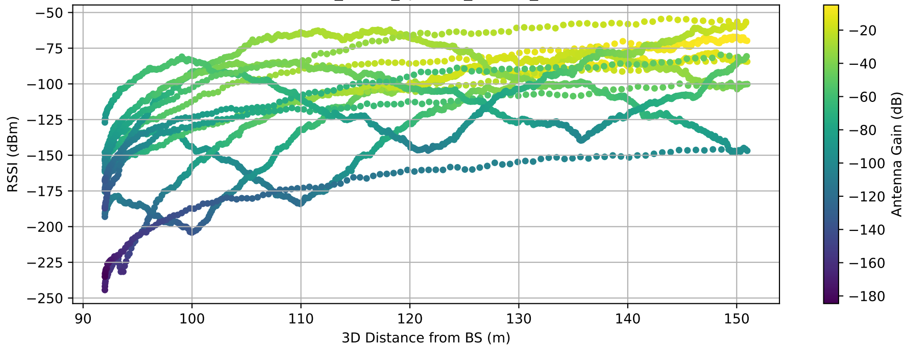
RSSI vs Distance — SPIRAL_6orbit_spc15m_alt95m_20260310T142457Z.csv
