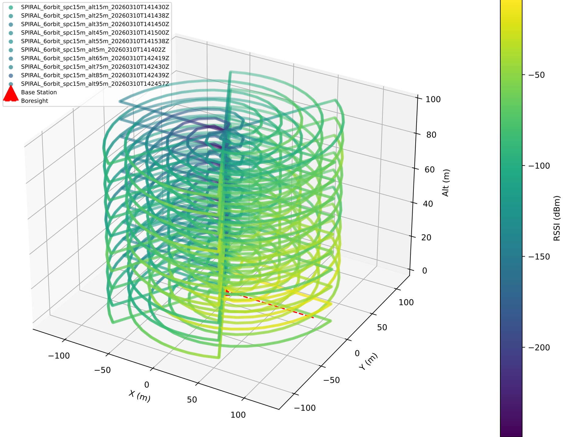
All Plans — 3D Paths by RSSI (10 plans)
