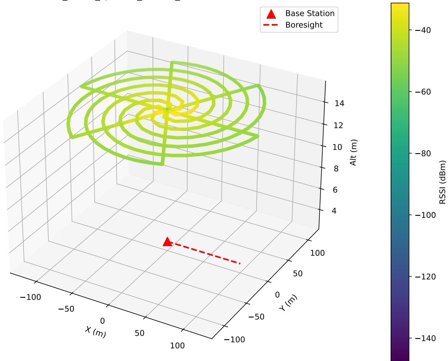
3D Path — RSSI (dBm) SPIRAL_6orbit_spc15m_alt15m_20260310T141430Z.csv
