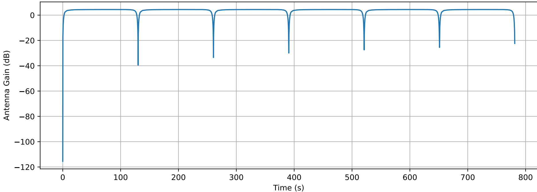
Antenna Gain Along Path — SPIRAL_6orbit_spc15m_alt15m_20260310T141430Z.csv
