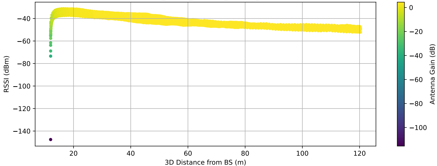
RSSI vs Distance — SPIRAL_6orbit_spc15m_alt15m_20260310T141430Z.csv
