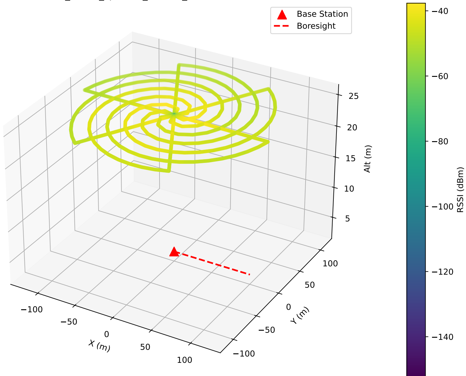
3D Path — RSSI (dBm) SPIRAL_6orbit_spc15m_alt25m_20260310T141438Z.csv
