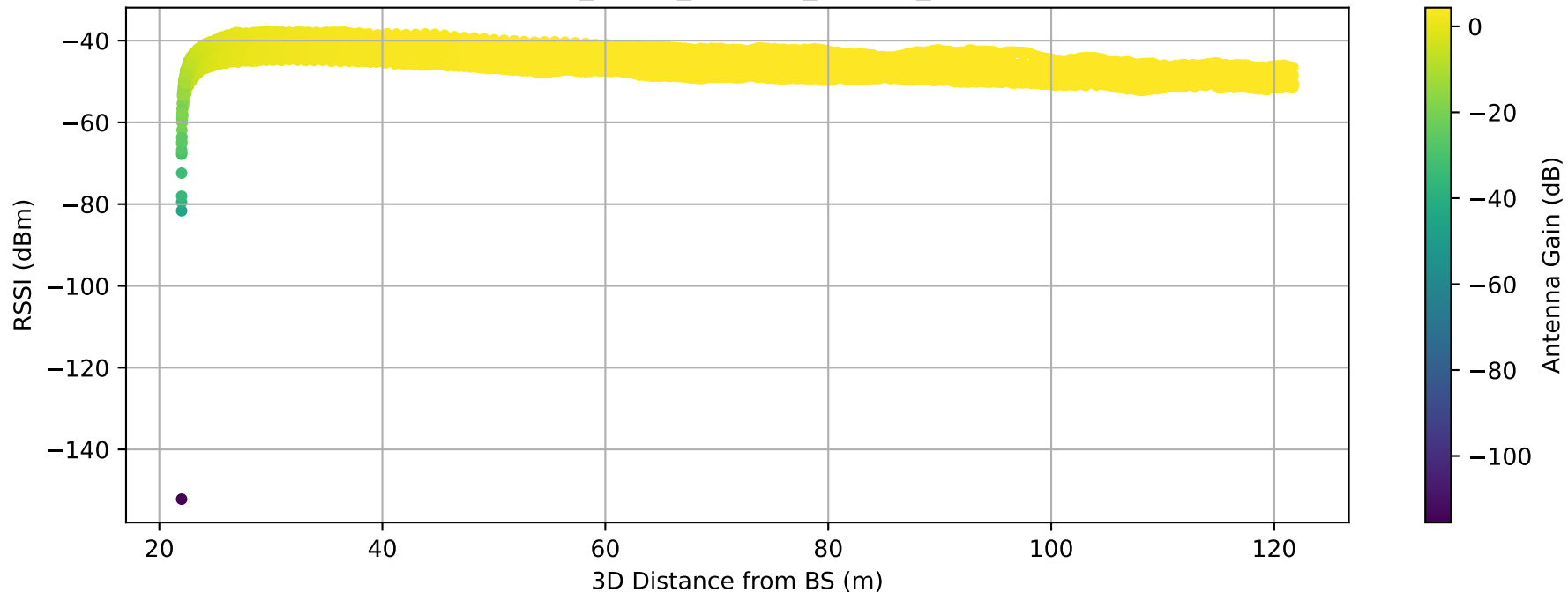
RSSI vs Distance — SPIRAL_6orbit_spc15m_alt25m_20260310T141438Z.csv
