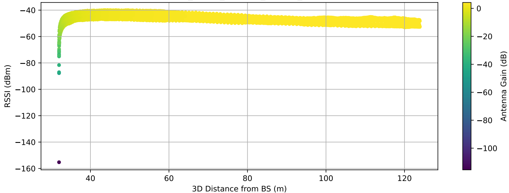
RSSI vs Distance — SPIRAL_6orbit_spc15m_alt35m_20260310T141450Z.csv
