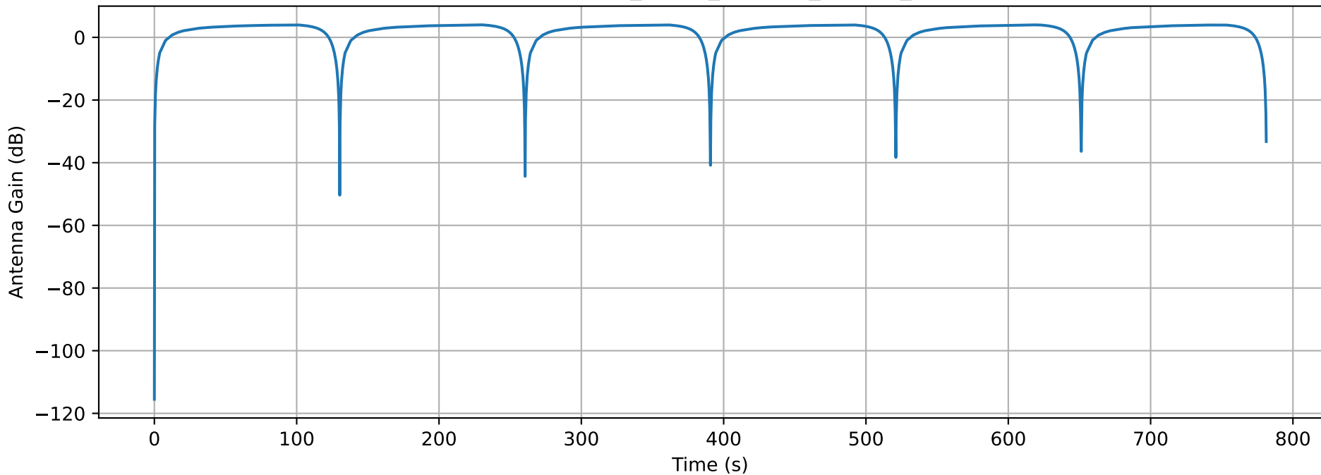
Antenna Gain Along Path — SPIRAL_6orbit_spc15m_alt45m_20260310T141500Z.csv
