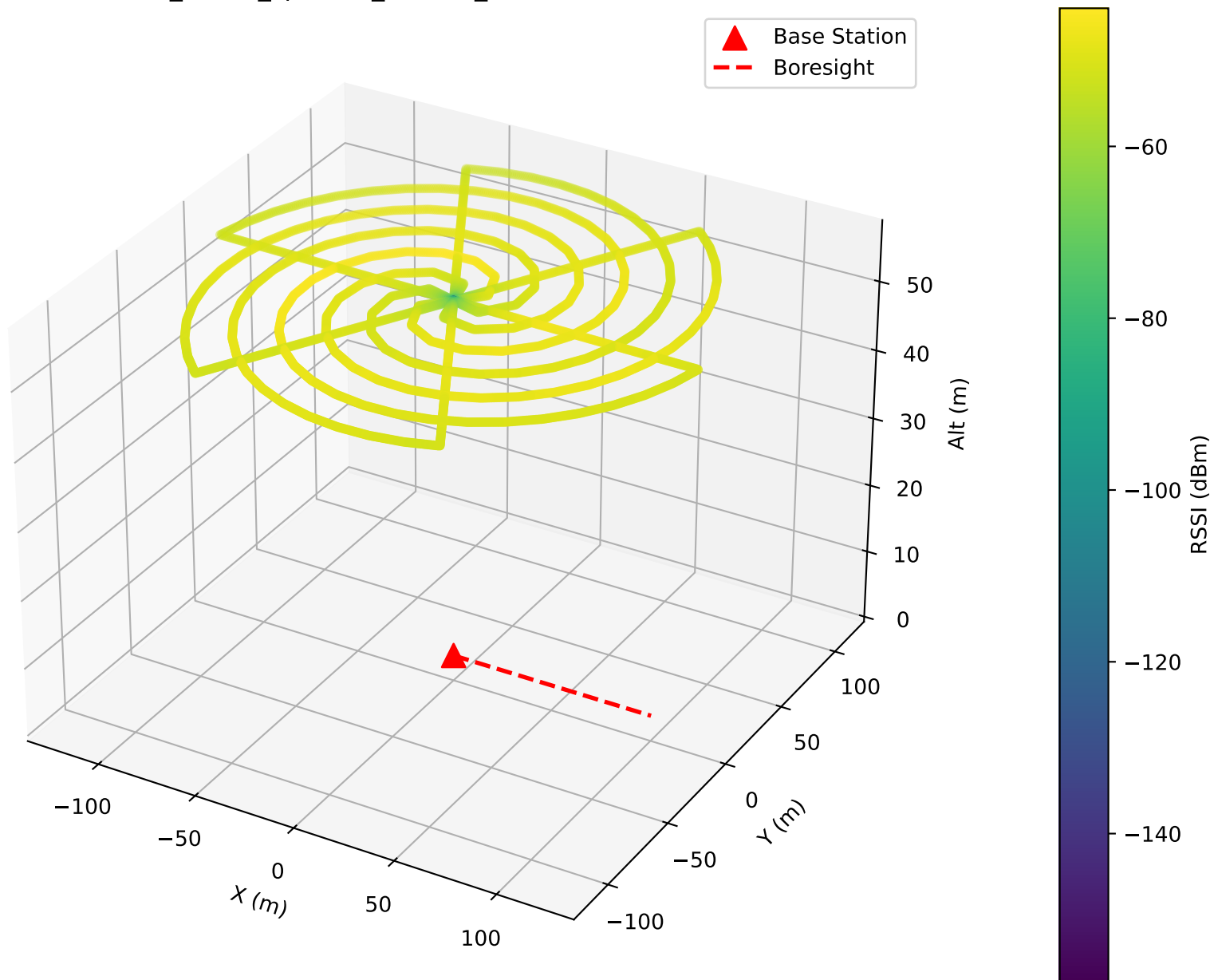
3D Path — RSSI (dBm) SPIRAL_6orbit_spc15m_alt55m_20260310T141538Z.csv
