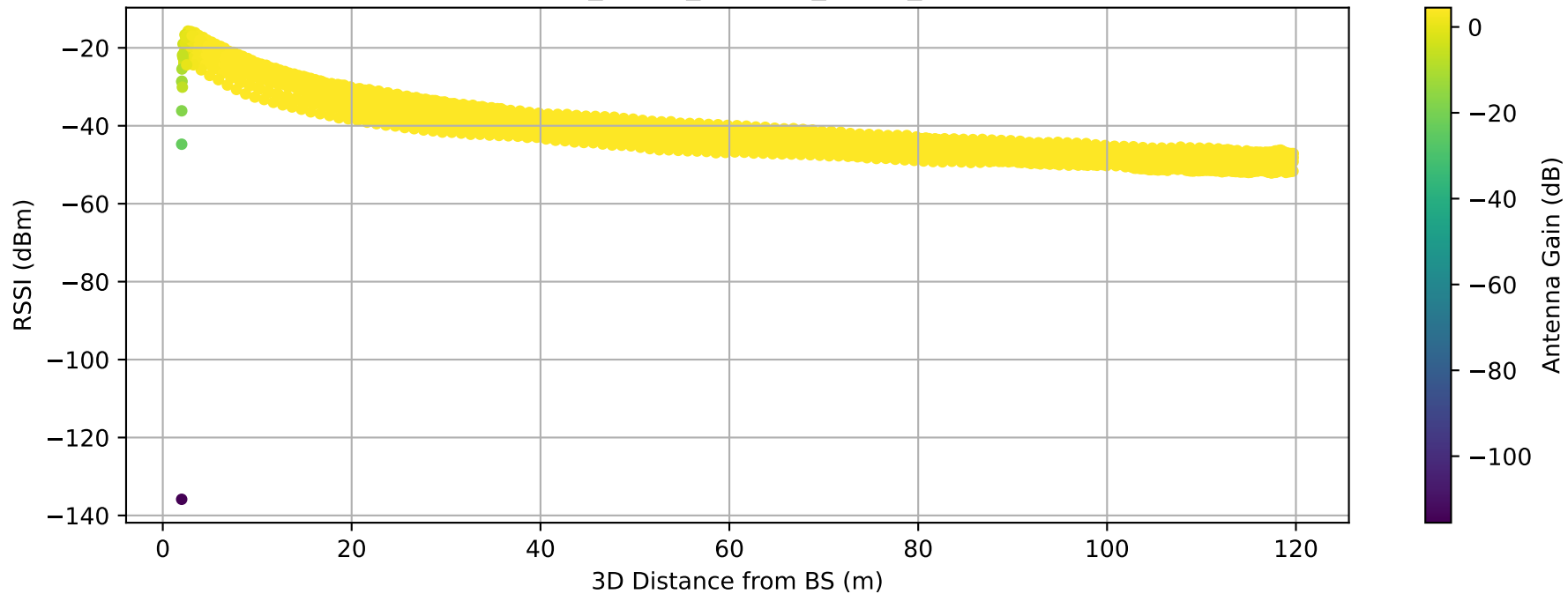
RSSI vs Distance — SPIRAL_6orbit_spc15m_alt5m_20260310T141402Z.csv
