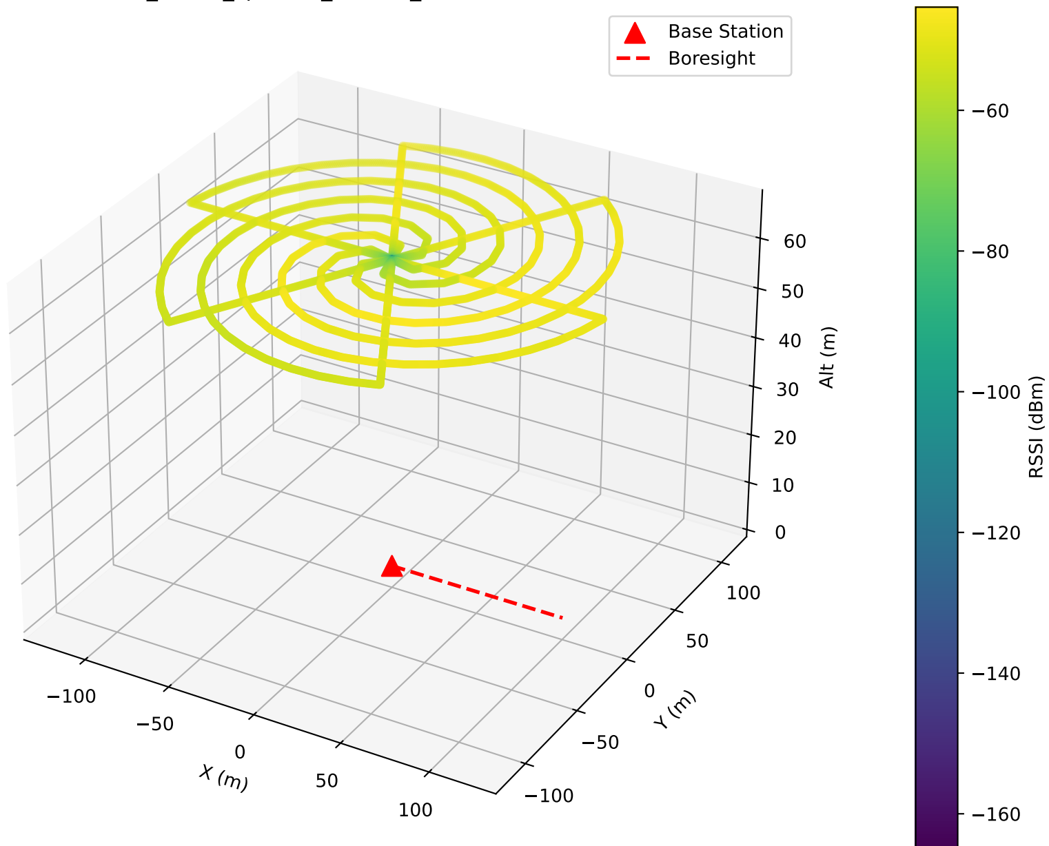
3D Path — RSSI (dBm) SPIRAL_6orbit_spc15m_alt65m_20260310T142419Z.csv
