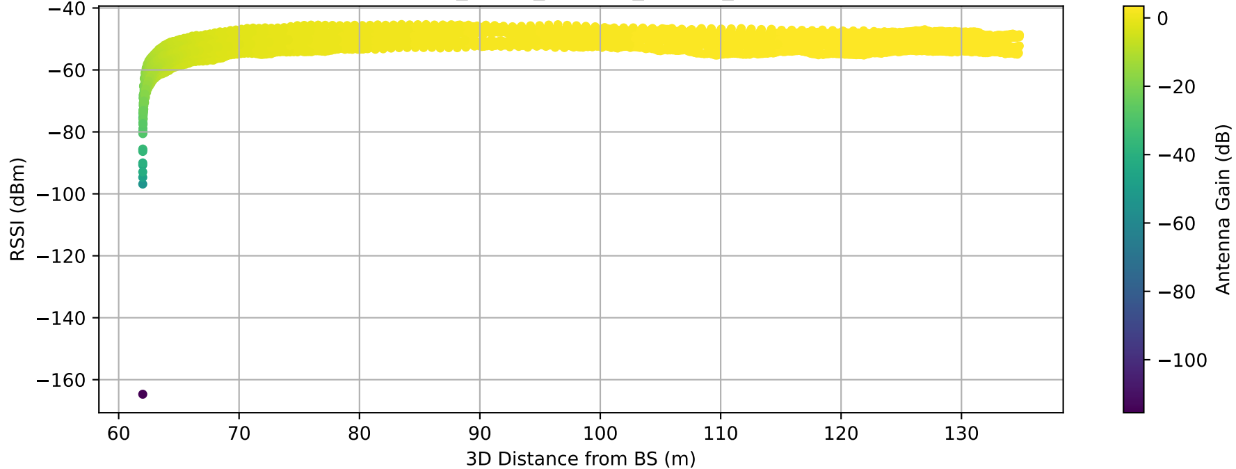
RSSI vs Distance — SPIRAL_6orbit_spc15m_alt65m_20260310T142419Z.csv
