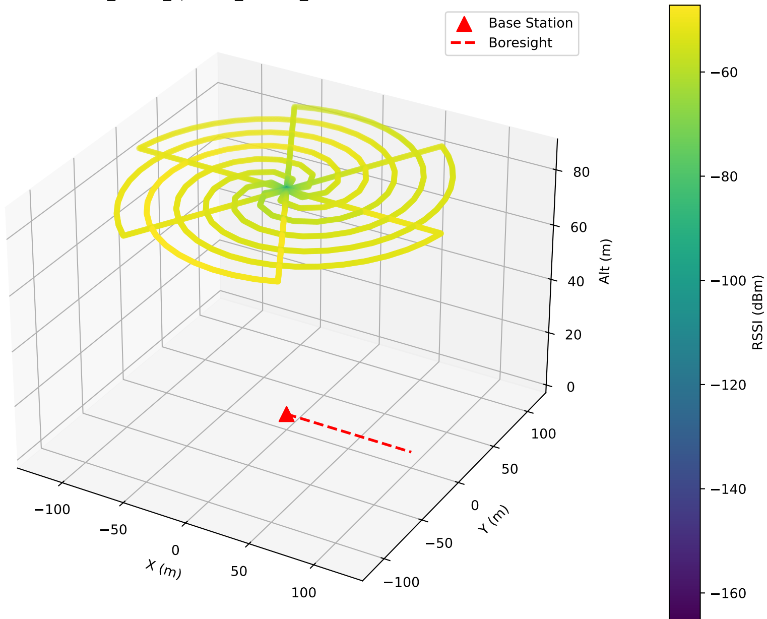
3D Path — RSSI (dBm) SPIRAL_6orbit_spc15m_alt85m_20260310T142439Z.csv
