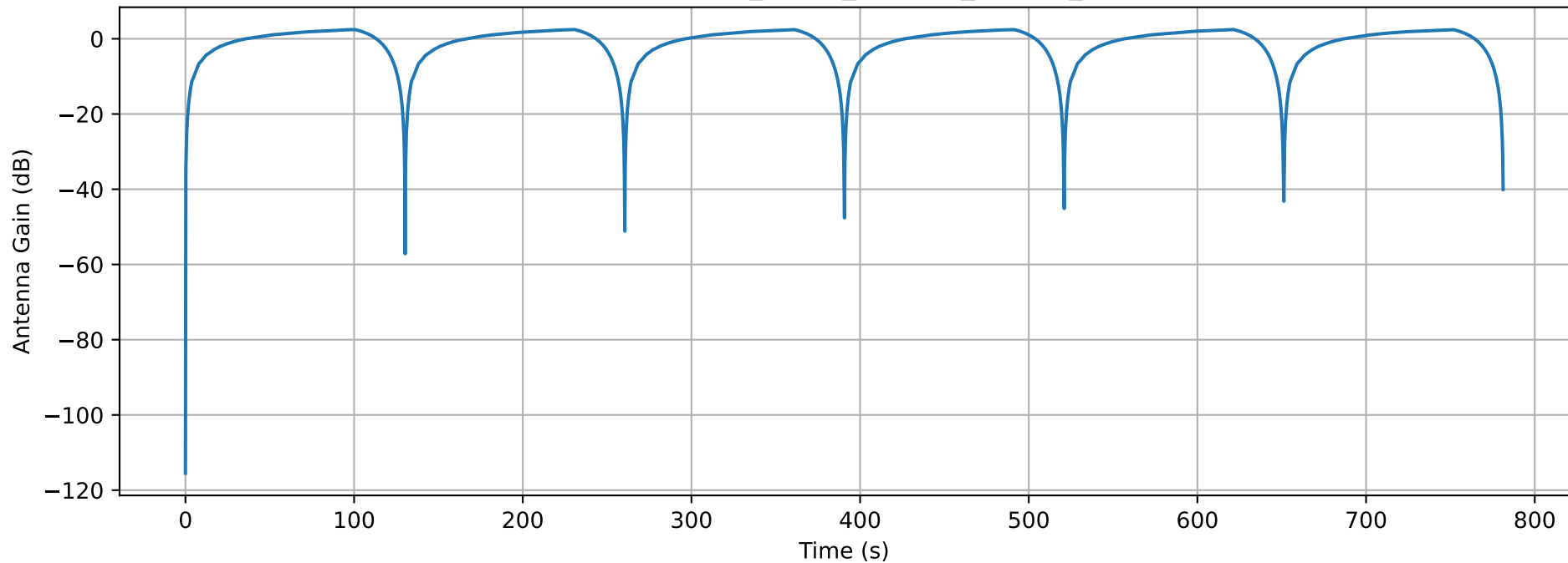
Antenna Gain Along Path — SPIRAL_6orbit_spc15m_alt95m_20260310T142457Z.csv
