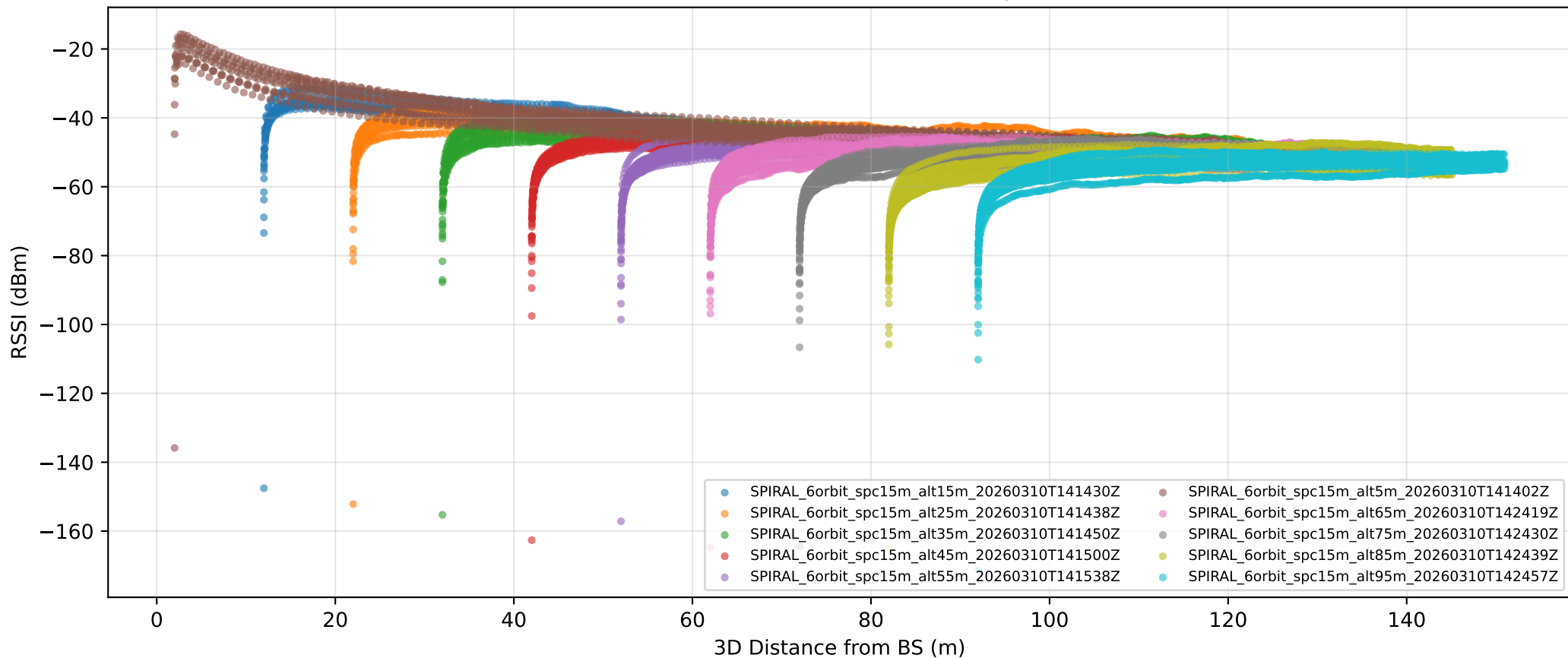
All Plans — RSSI vs Distance (10 plans)
