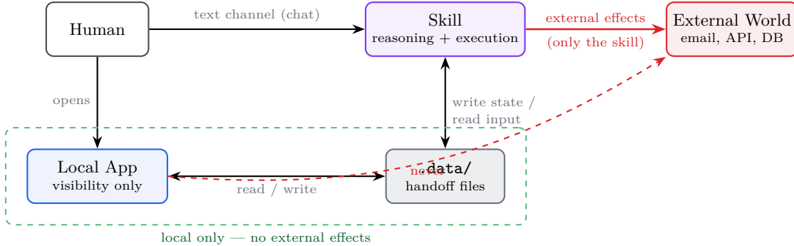
Figure 3: The two channels and the boundary. The human reaches one skill through two channels: the text channel (chat) and the local app. The app and the handoff files ( .data/ ) live in a local-only zone; the skill is the only component that produces external effects (red). The app never reaches the external world.
