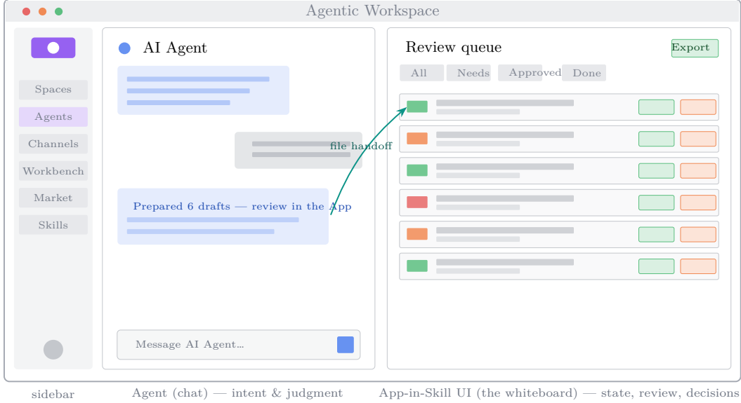
Figure 2: A typical App-in-Skill layout in an agentic workspace (e.g. Claude Code, Codex, Buda AI). A navigation sidebar (left), the agent chat (middle), and the App-in-Skill UI (right) are on screen together. The agent prepares work in chat and hands it to the app through a file handoff (teal); the human reviews, edits, and decides in the app’s queue (status badges, action buttons), then returns to chat for judgment. The app does not replace the conversation—it is the whiteboard the conversation reaches for.
