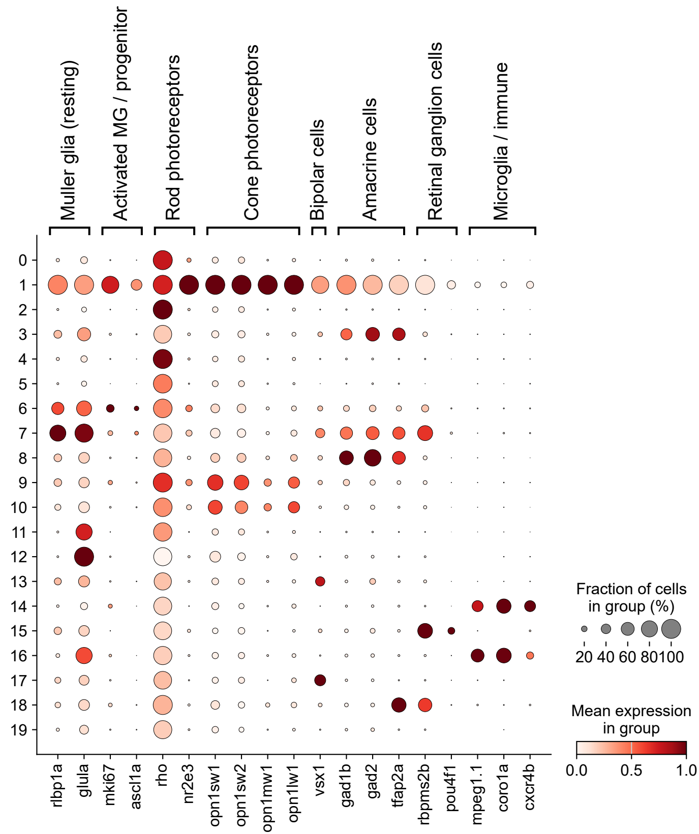
Figure 3A | Canonical marker expression
