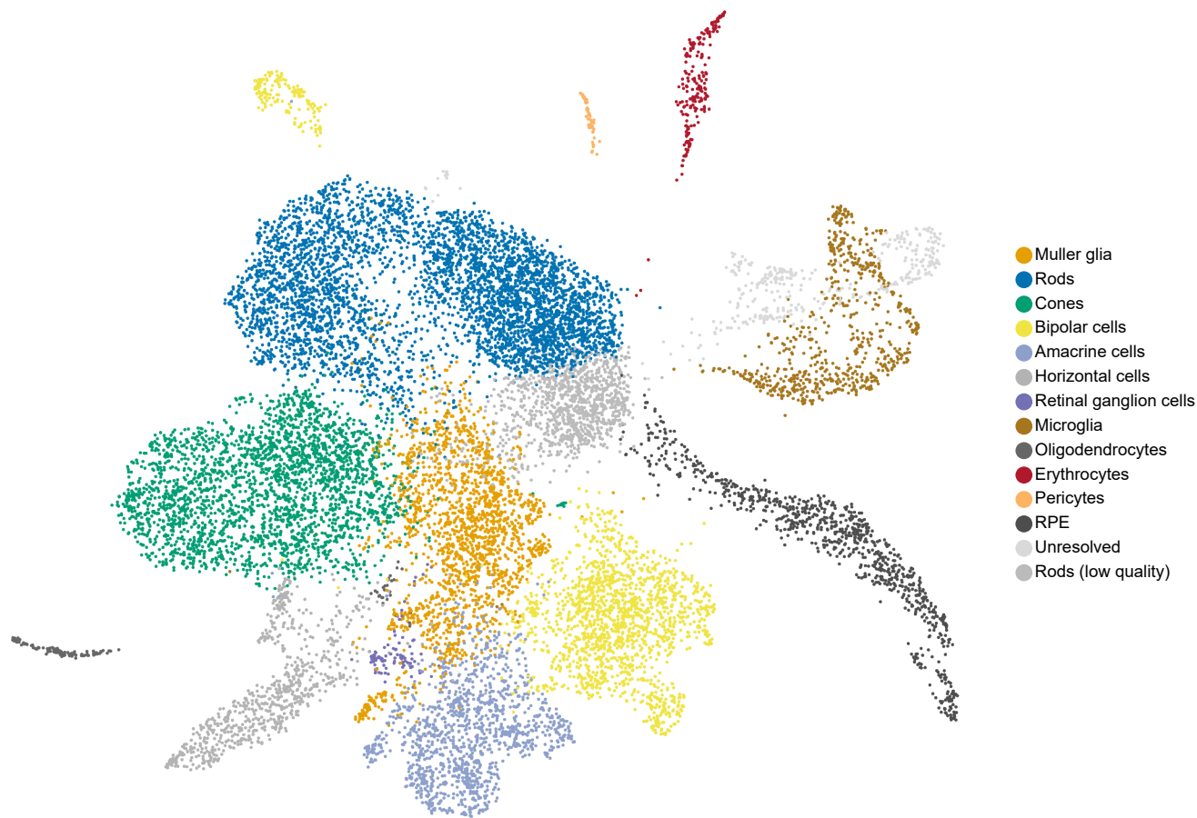
Fig 5C equivalent | cell populations
