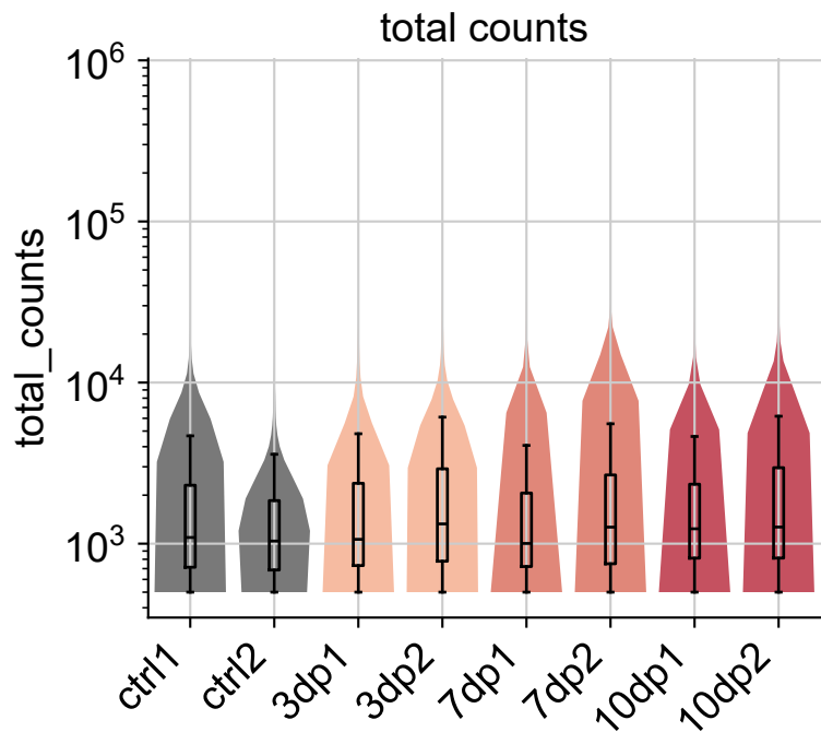
Figure 1 | Quality control across the eight samples
