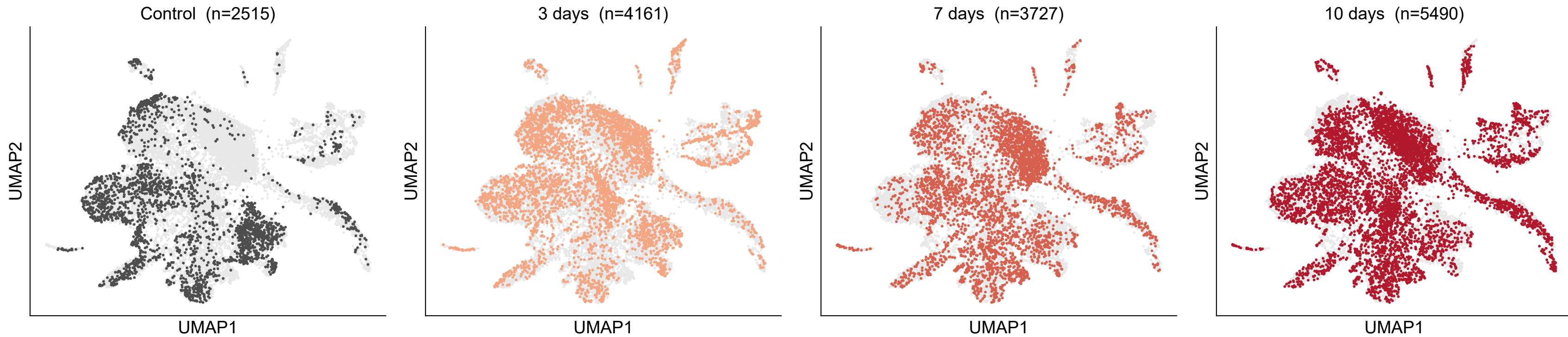
Figure 2D | Cells by timepoint on the shared embedding
