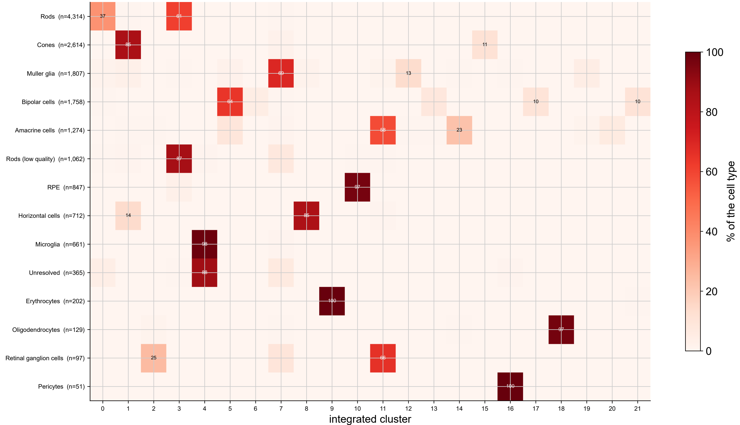
Integration sensitivity | where each annotated cell type went (row-normalised %; a row confined to one column survived intact)
