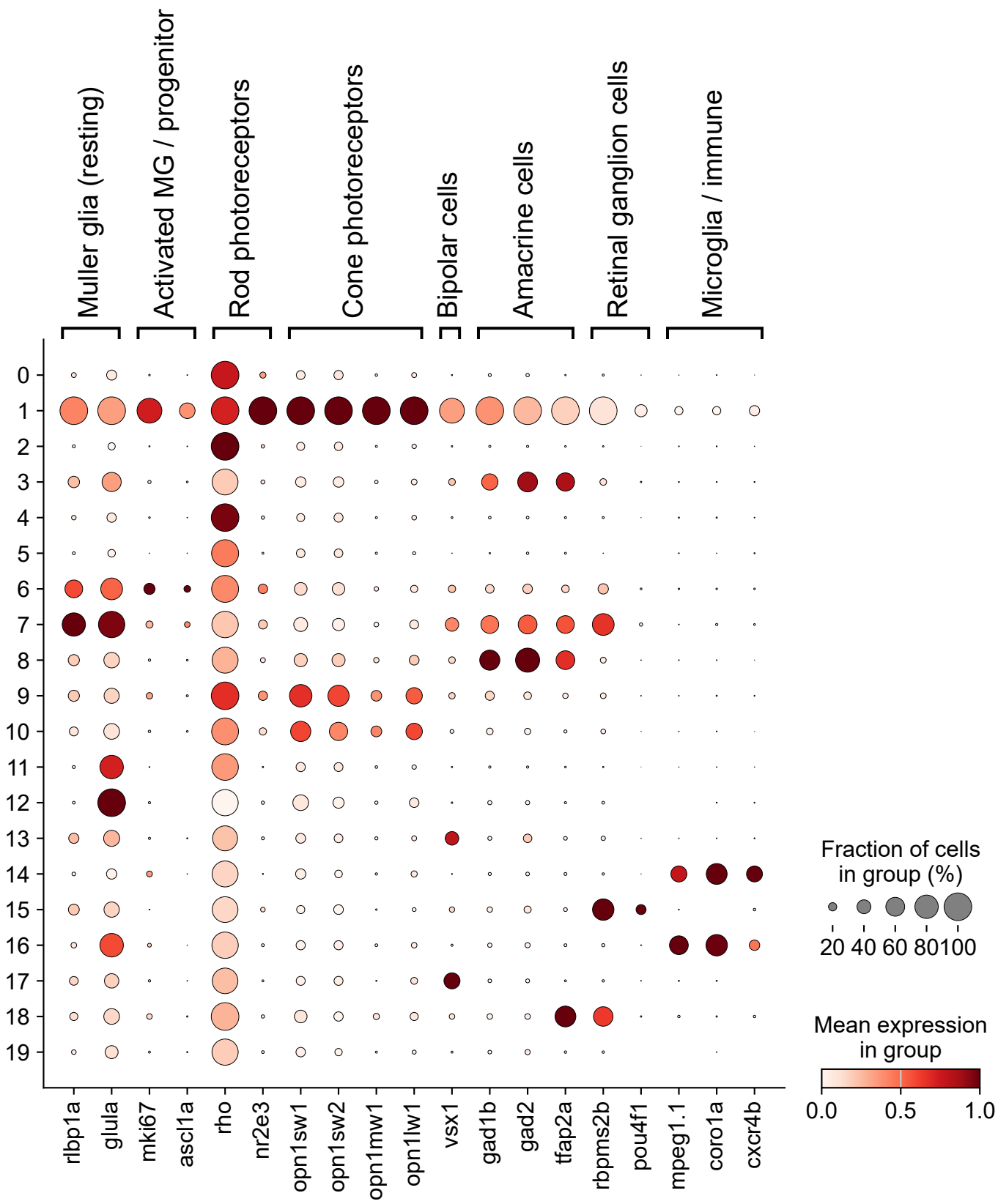
Figure 3A | Canonical marker expression
