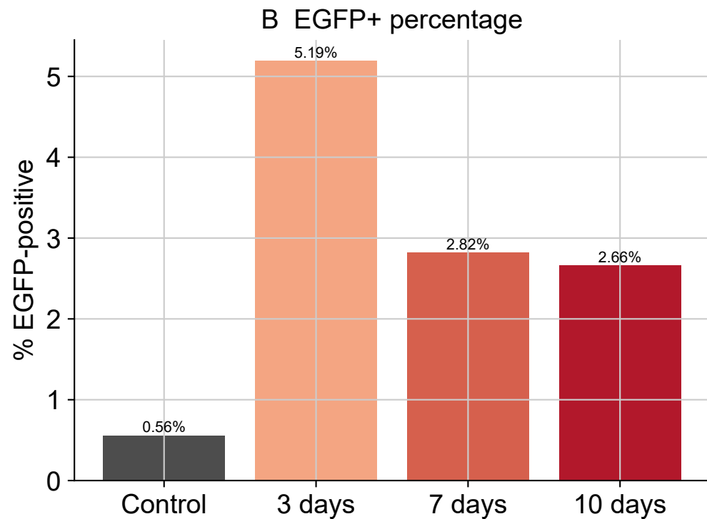
Fig 8B equivalent | EGFP-positive cells across the time course
