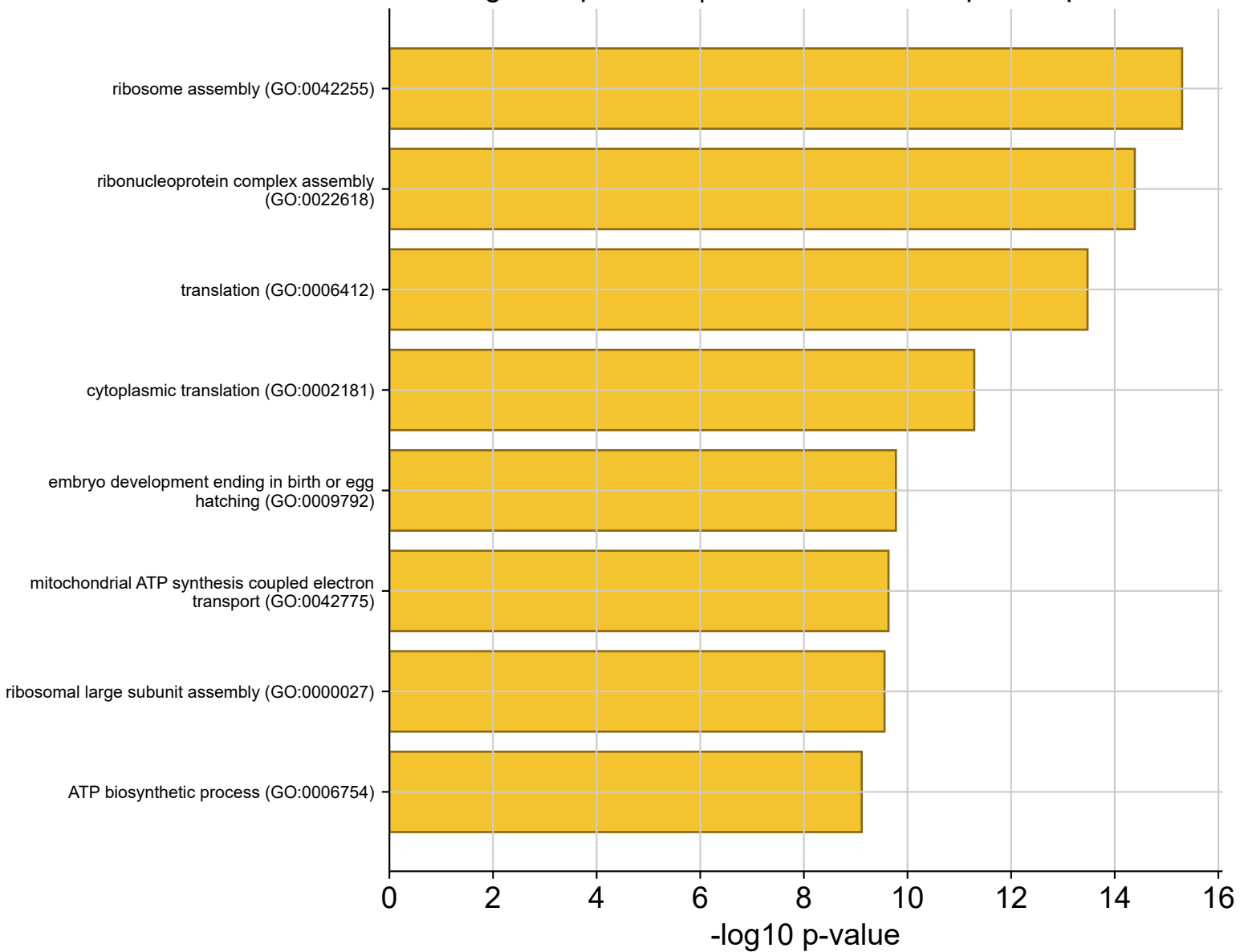
Fig 7F equivalent | GO terms, cones up at 3 dpMNU
