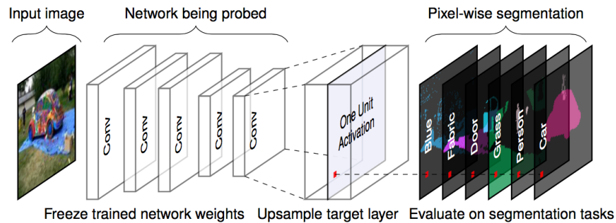
FIGURE 9.5 For a given input image and a trained network (fixed weights), we propagate the image forward to the target layer, upscale the activations to match the original image size and compare the maximum activations with the ground truth pixel-wise segmentation. Figure originally from the [project website]( http://netdissect.csail.mit.edu/ ).
