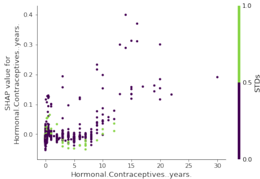
FIGURE 8.28 SHAP feature dependence plot with interaction visualization. Years on hormonal contraceptives interacts with STDs. In cases close to 0 years, the occurrence of a STD increases the predicted cancer risk. For more years on contraceptives, the occurrence of a STD reduces the predicted risk. Again, this is not a causal model. Effects might be due to confounding (e.g. STDs and lower cancer risk could be correlated with more doctor visits).
