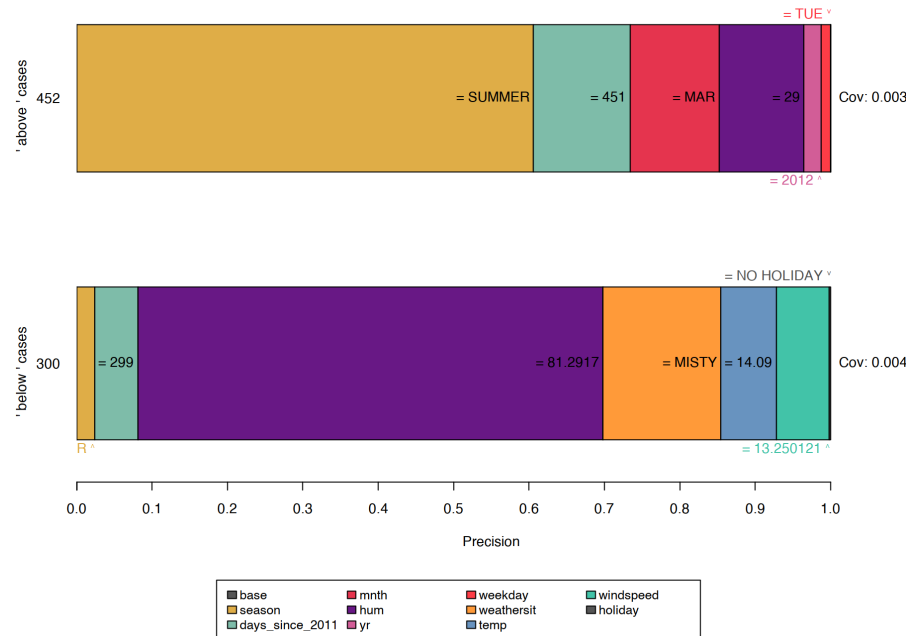
FIGURE 8.14 Explaining instances near decision boundaries leads to specific rules comprising a higher number of feature predicates and lower coverage. Also, the empty rule, i.e. the base feature, gets less important. This can be interpreted as a signal for a decision boundary, as the instance is located in a volatile neighborhood.
