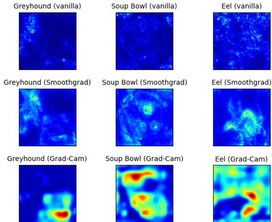
FIGURE 9.10 Pixel attributions or saliency maps for the Vanilla Gradient method, SmoothGrad and Grad-CAM.
