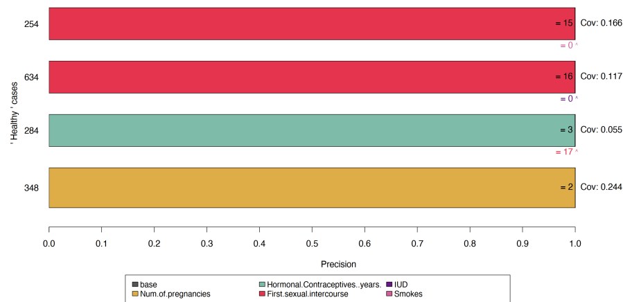
FIGURE 8.16 Balancing the data set before constructing anchors shows the model's reasoning for decisions in minority cases.
