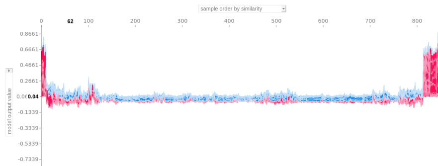
FIGURE 8.29 Stacked SHAP explanations clustered by explanation similarity. Each position on the x-axis is an instance of the data. Red SHAP values increase the prediction, blue values decrease it. One cluster stands out: On the right is a group with a high predicted cancer risk.
