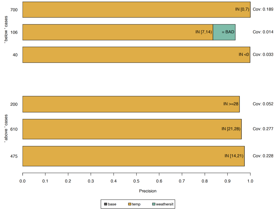
FIGURE 8.13 Anchors explaining six instances of the bike rental dataset. Each row represents one explanation or anchor, and each bar depicts the feature predicates contained by it. The x-axis displays a rule's precision, and a bar's thickness corresponds to its coverage. The "base" rule contains no predicates. These anchors show that the model mainly considers the temperature for predictions.
