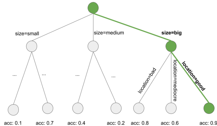
FIGURE 4.20 Learning a rule by searching a path through a decision tree. A decision tree is grown to predict the target of interest. We start at the root node, greedily and iteratively follow the path which locally produces the purest subset (e.g. highest accuracy) and add all the split values to the rule condition. We end up with: If ‘location=good’ and ‘size=big’, then ‘value=high’.
