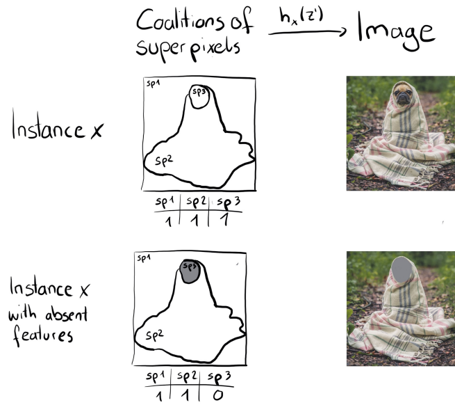
FIGURE 8.23 Function h_x maps coalitions of superpixels (sp) to images. Superpixels are groups of pixels. For present features (1), h_x returns the corresponding part of the original image. For absent features (0), h_x greys out the corresponding area. Assigning the average color of surrounding pixels or similar would also be an option.
