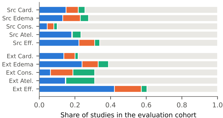
Impression-derived labels
