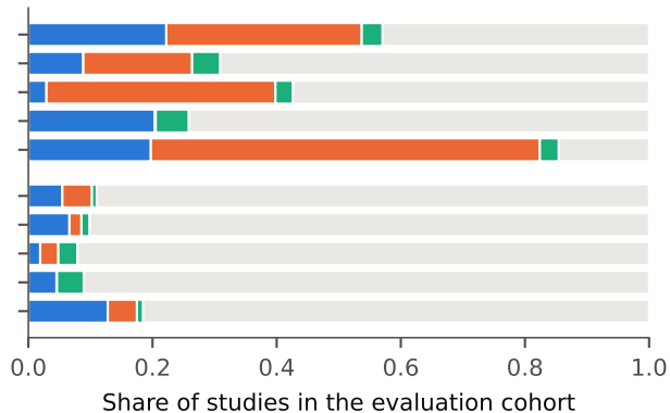
Findings-derived labels
