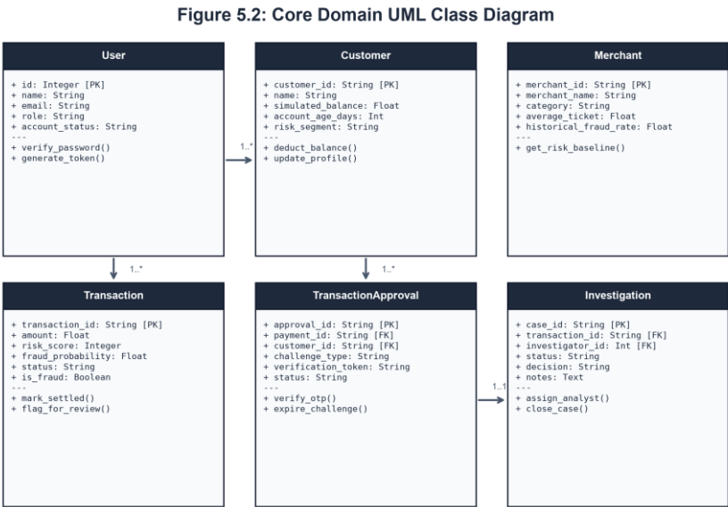
Figure 5.2: Core Domain UML Class Diagram
