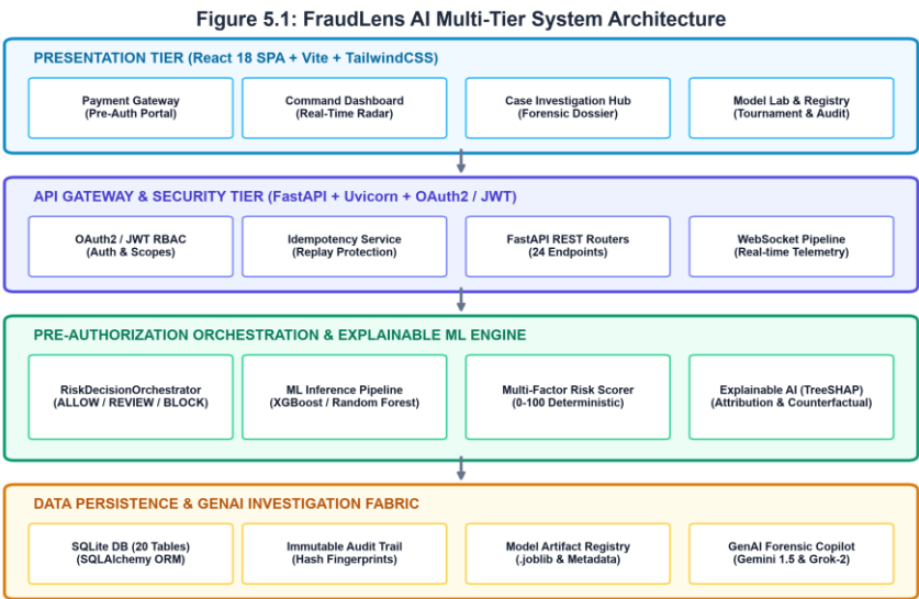
Figure 5.1: FraudLens AI Multi-Tier System Architecture
