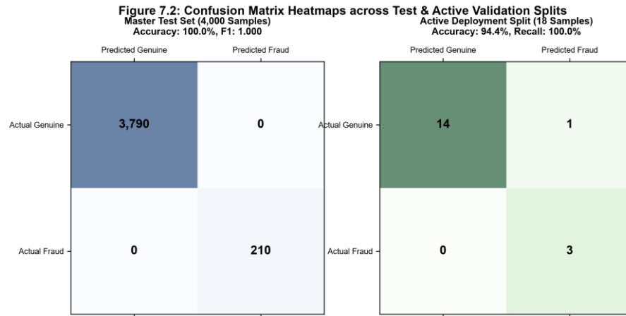
Figure 7.2: Confusion Matrix Heatmaps across Test & Active Validation Splits
