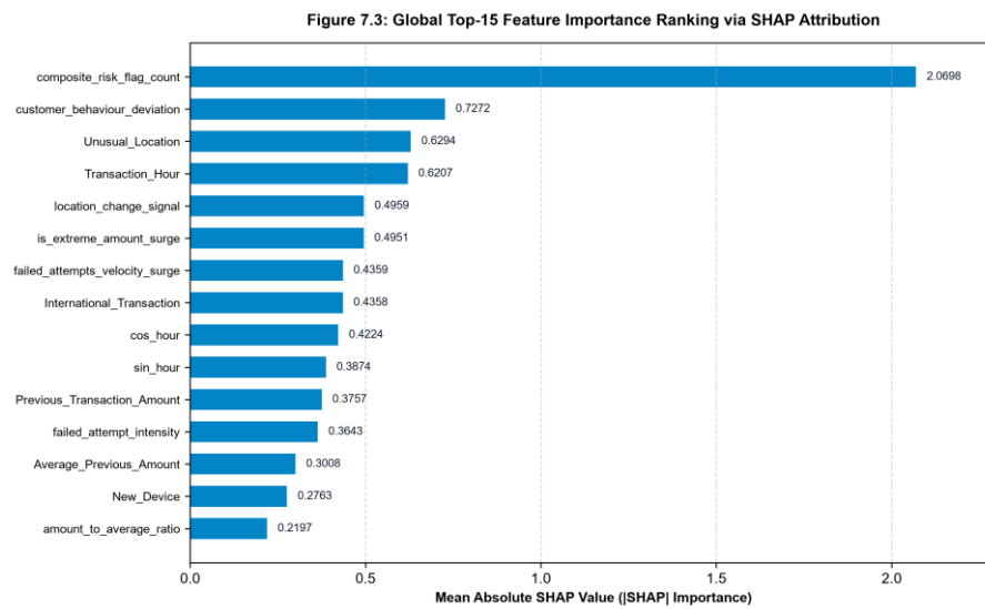
Figure 7.3: Global Top-15 Feature Importance Ranking via TreeSHAP
