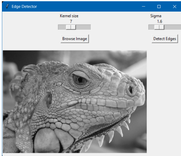
Figure 1. Iguana GUI
