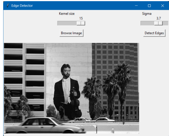
Figure 2. Building GUI
