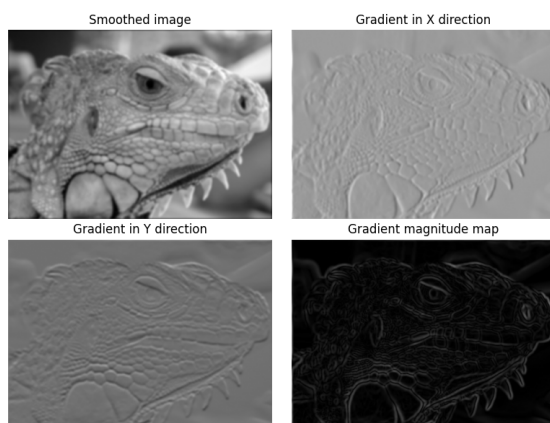
Figure 3. Iguana Results
