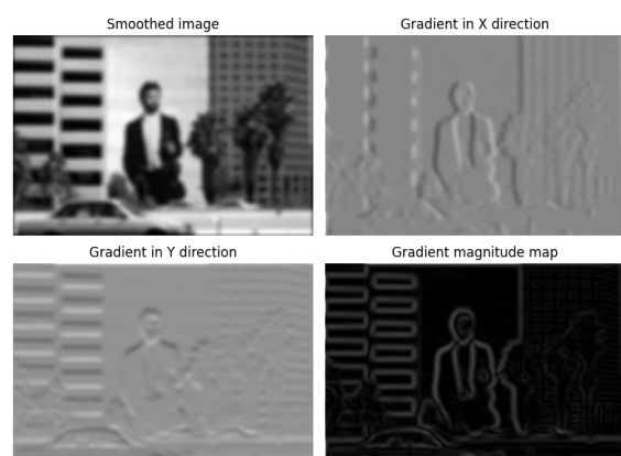
Figure 4. Building Results
