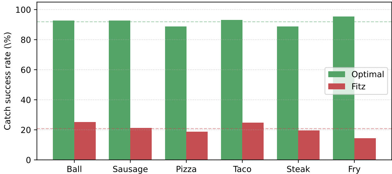
Catch success rate per object (n = 1000 throws per dog)
