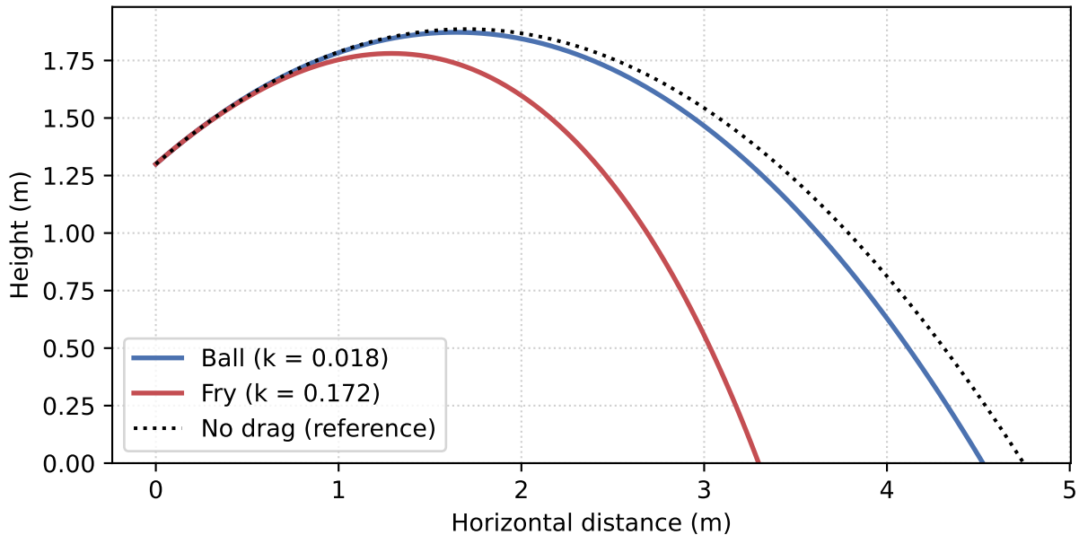
Trajectories for a 6.0 m/s launch at 35° from height 1.3 m
